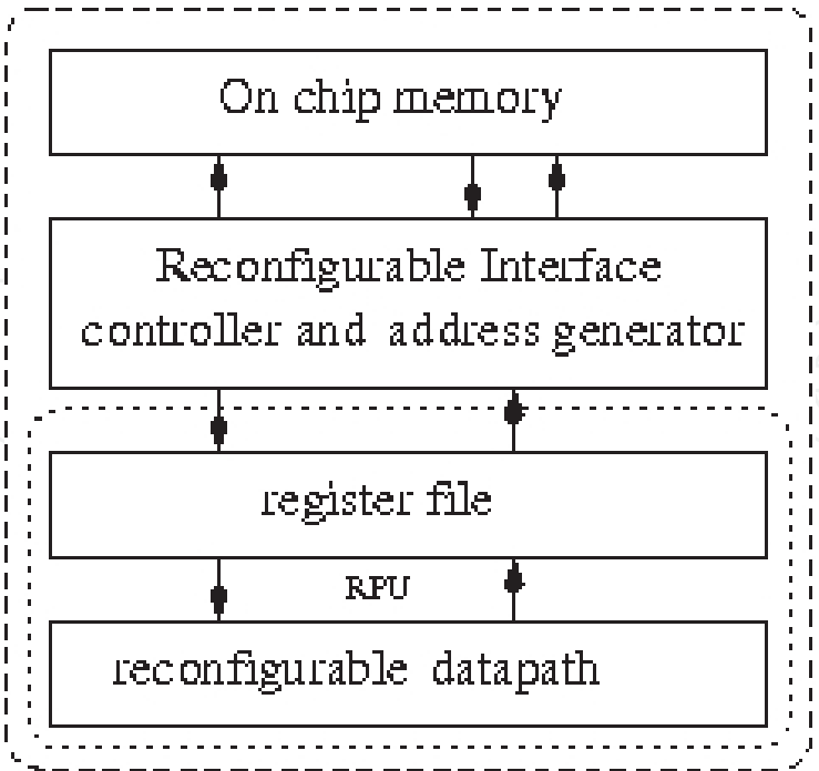
Fig. 5. General architecture of a RPU
