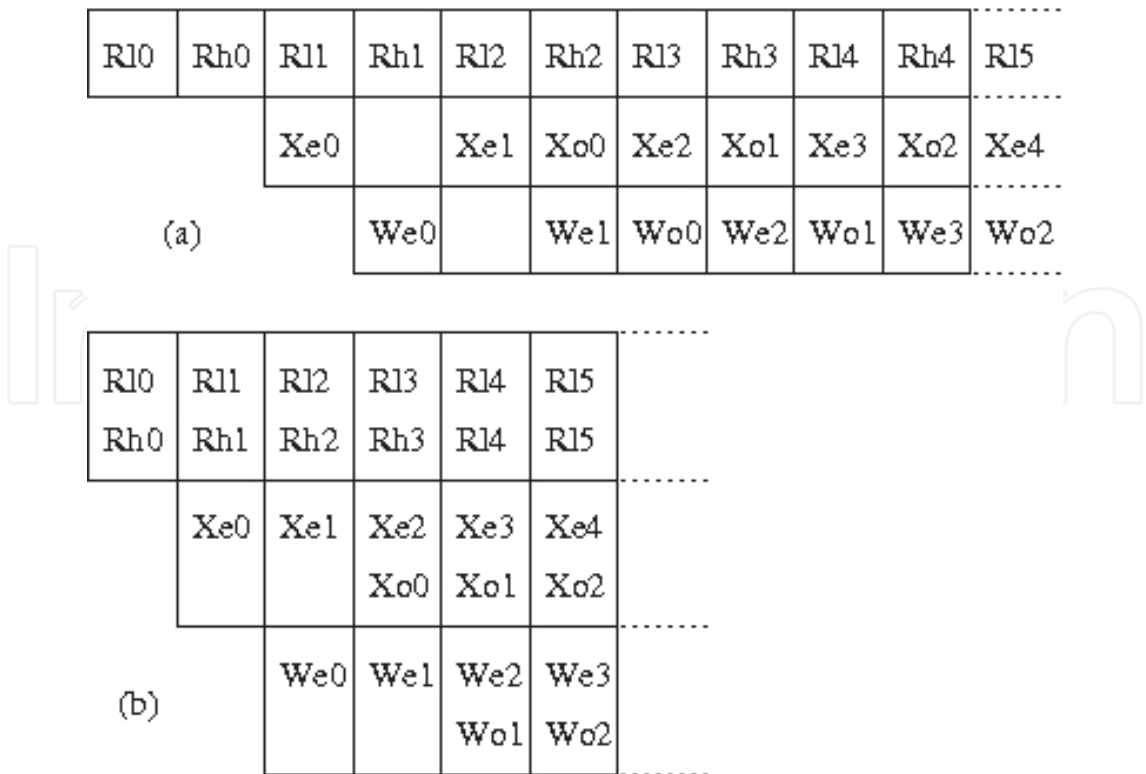
Fig. 7. Pipeline organization: special case (a) and normal case(b)
