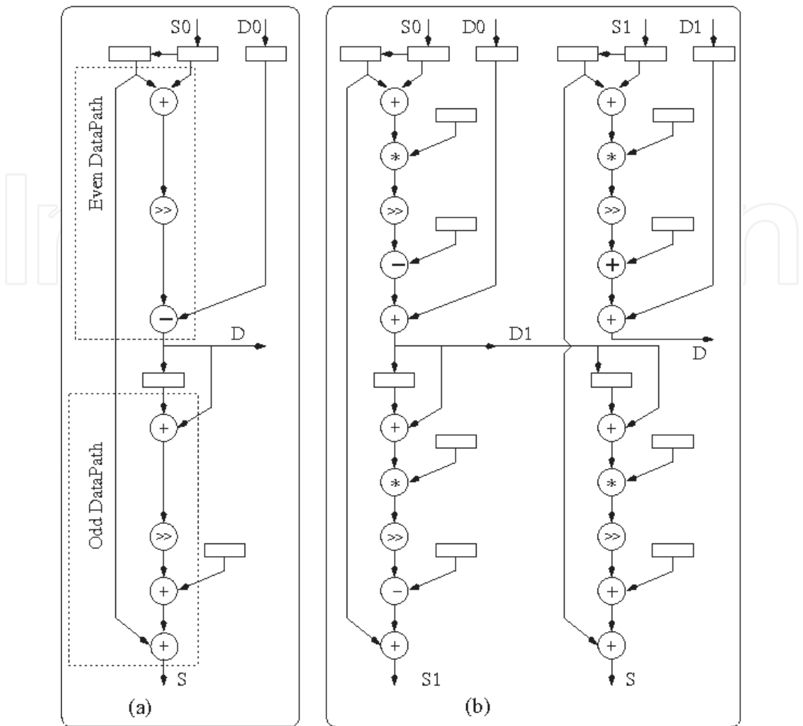
Fig. 6. IDWT 5/3 (a) and 9/7 DFG (b)
