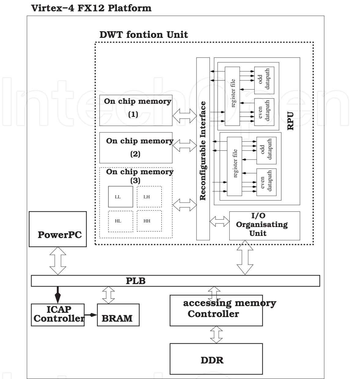
Fig. 9. Target architecture.
