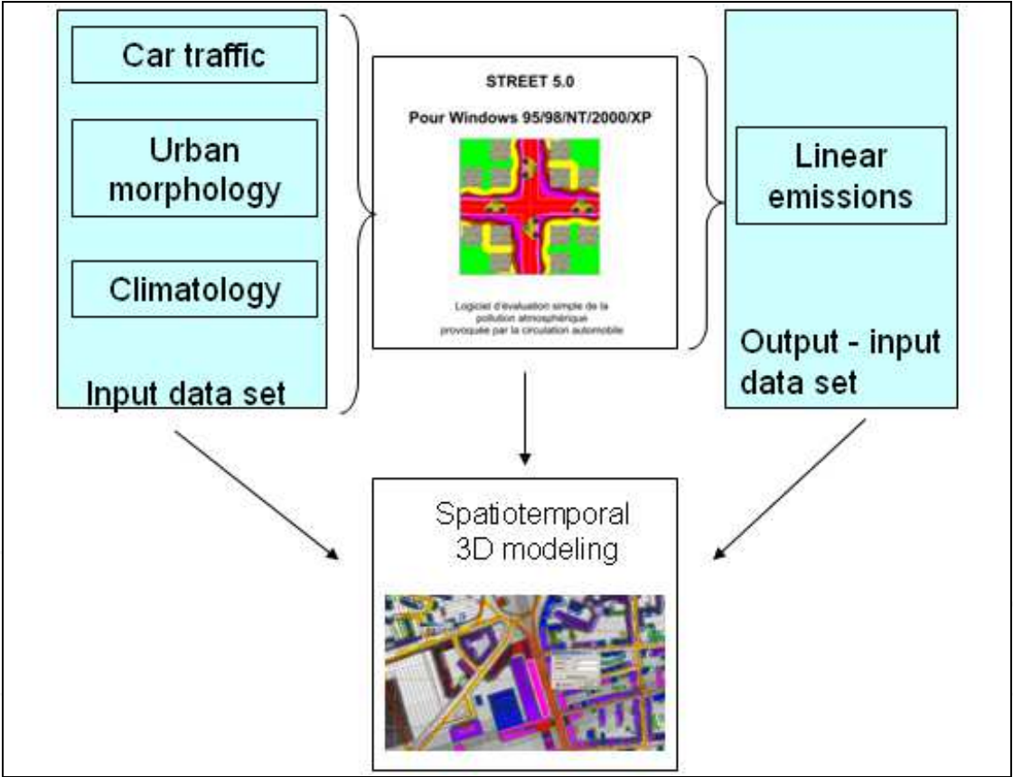
Fig. 2. Air pollution modelling, from sources to maps.
