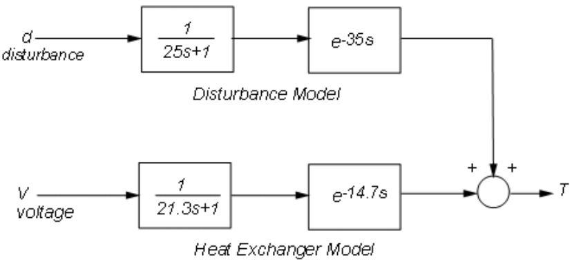
Fig. 13. Open loop process model The transfer function
