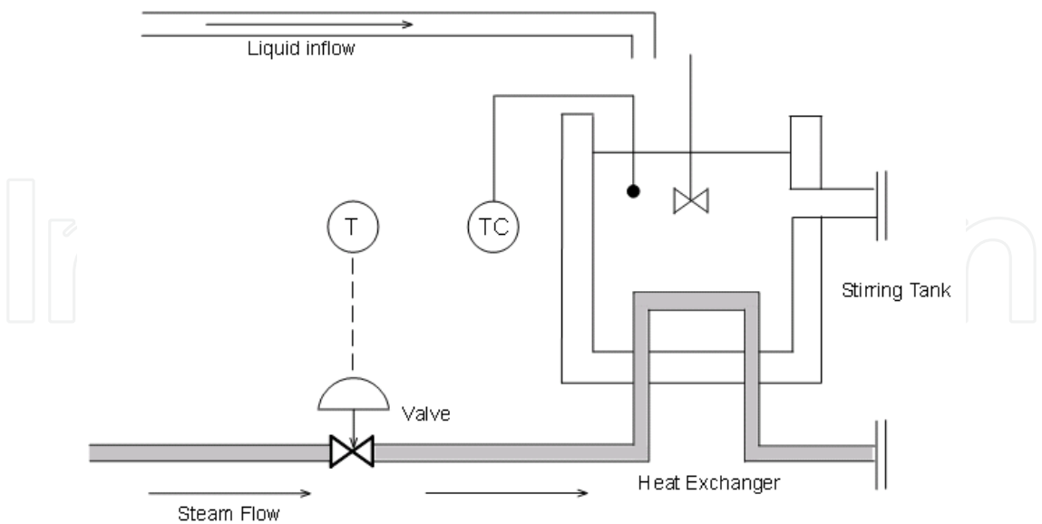
Fig. 12. Stirring Reactor with Heat Exchanger The process can be modelled adequately by FOPDT models as shown in the Fig. 13.
