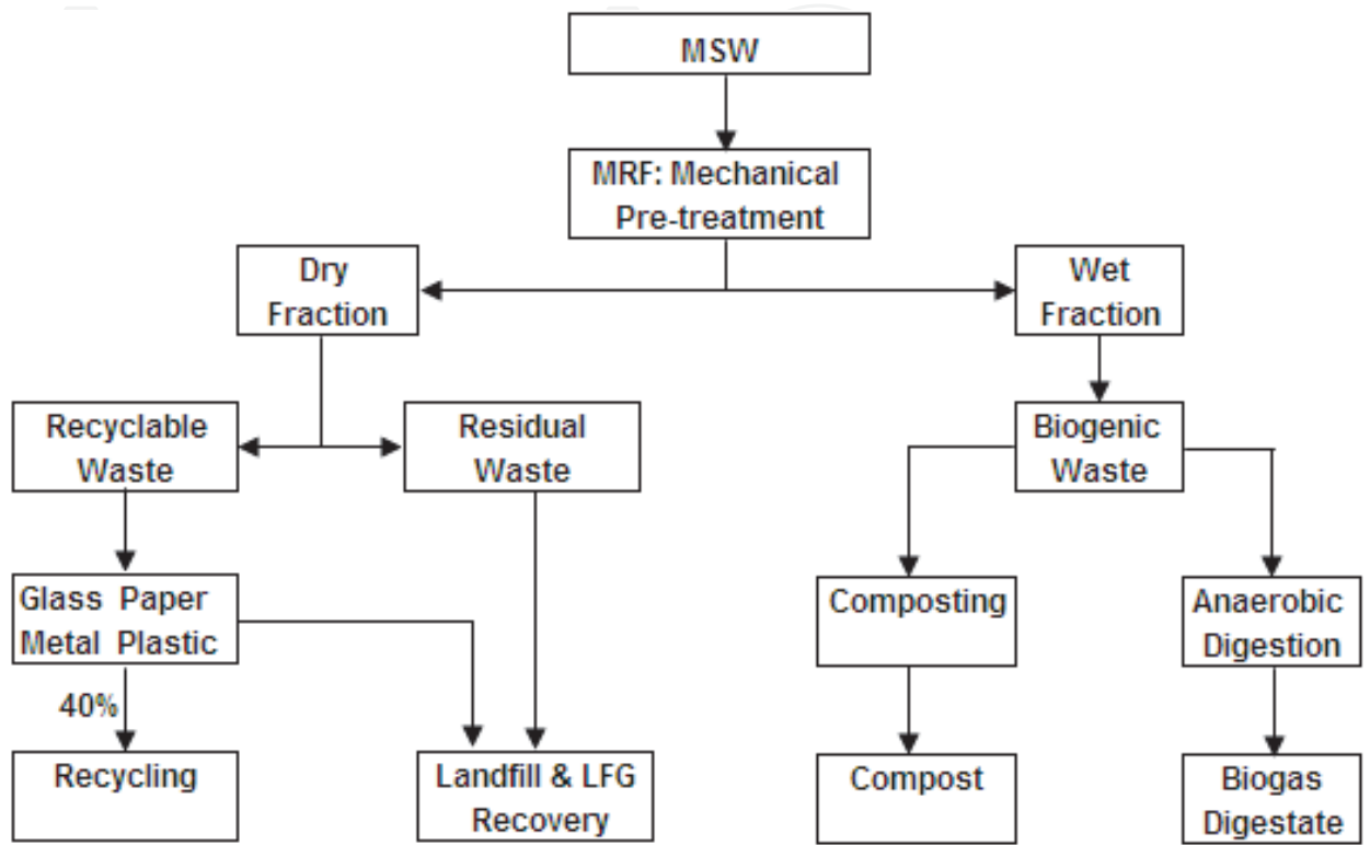
Fig. 1. A typical dry-wet waste diversion model (Matete and Trois, 2008; Trois and Simelane, 2010)
