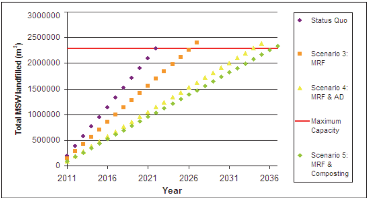
Fig. 6. Predicted airspace capacity trends: Mariannhill Landfill Site
