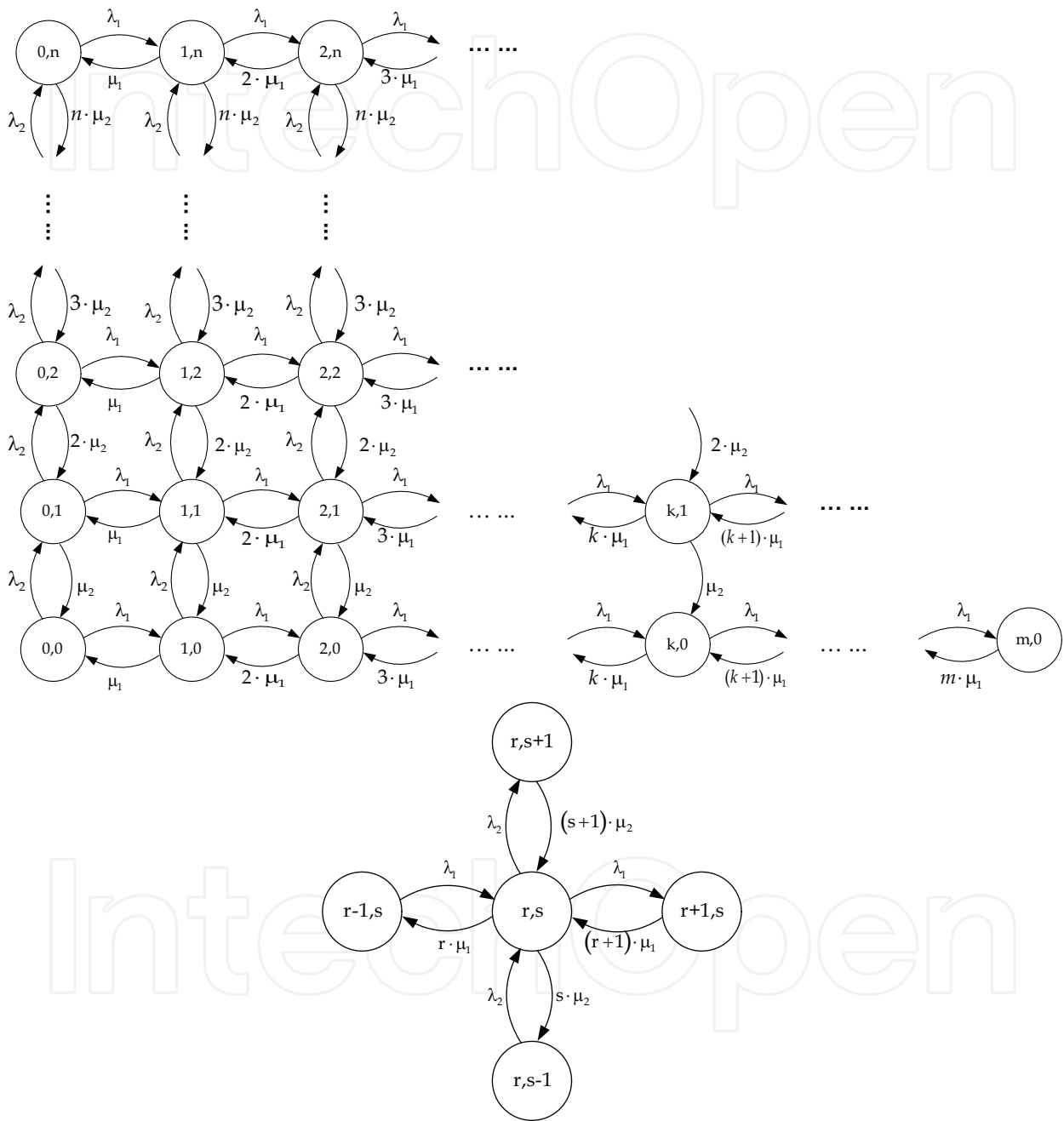
Fig. 3. The two-dimensional Markov model's state transition diagram Thus, the 2-dimensional continuous Markov model (Fig. 3) can be used to analyze the performance of the proposed scheme. The state space of this Markov model is
