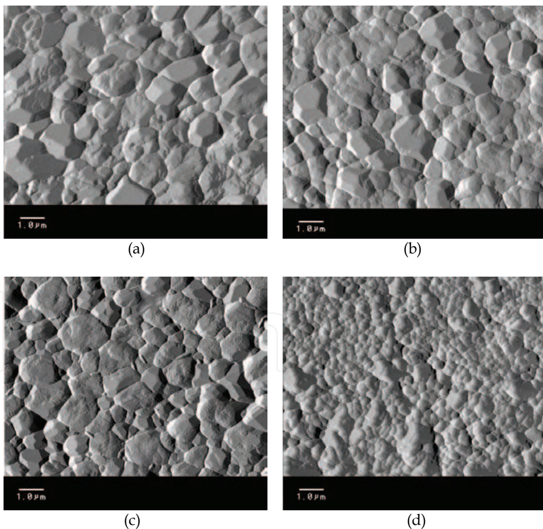
Fig. 13. Micrographies for (a) BZT10, (b) BZT10:1W, (c) BZT10:2W and (d) BZT10:4W ceramics prepared from mixed oxide method, sintered at 1200^{\circ}\text{C} for 4 hours.
