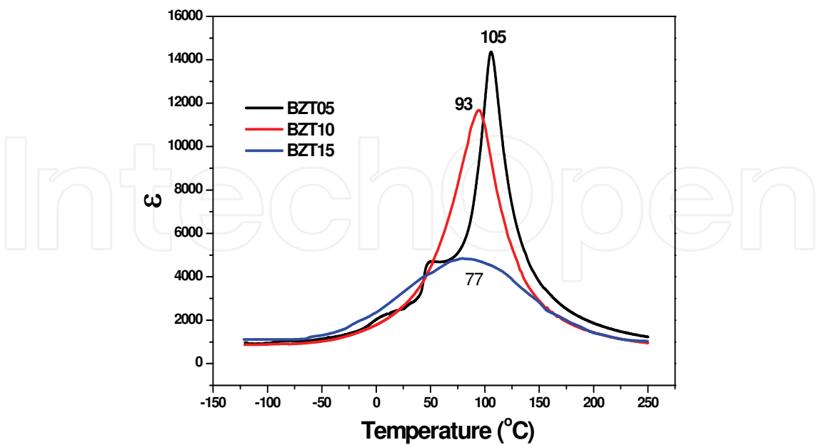
Fig. 5. Temperature dependence of dielectric permittivity ( \epsilon ) for BZT pellets with different concentrations, sintered at 1550 °C/4h: (a) Ba(Ti 0.95 Zr 0.05 )O 3 ; (b) Ba(Ti 0.9 Zr 0.10 )O 3 and (c) Ba(Ti 0.85 Zr 0.15 )O 3 .
