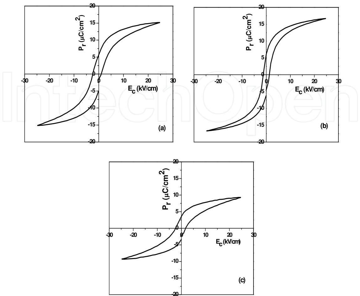
Fig. 6. P-E hysteresis loops for BZT pellets sintered at 1550 °C for 4 h in different concentrations: (a) Ba(Ti 0.95 Zr 0.05 )O 3 ; (b) Ba(Ti 0.9 Zr 0.10 )O 3 and (c) Ba(Ti 0.85 Zr 0.15 )O 3 .
