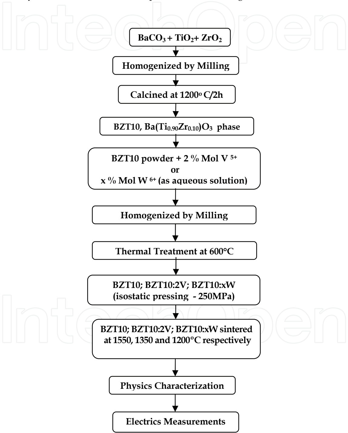
Fig. 1. Flowchart of the synthesis and characterization process of BZT10; BZT10:xV; BZT10:yW
