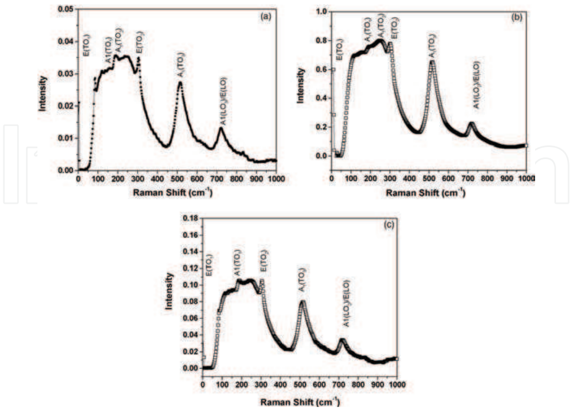
Fig. 4. Room temperature depolarized Raman spectra for BZT powders with different concentrations calculated at 1200°C for 2h: (a) Ba(Ti 0.95 Zr 0.05 )O 3 ; (b) Ba(Ti 0.9 Zr 0.10 )O 3 and (c) Ba(Ti 0.85 Zr 0.15 )O 3 .
