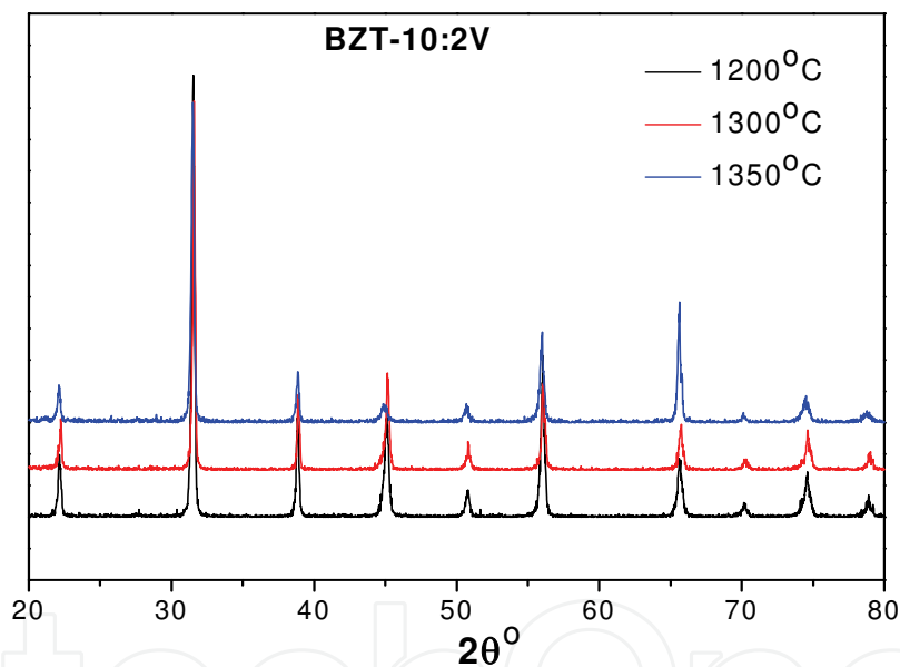
Fig. 7. X-ray diffraction of BZT10 and BZT10:xV ceramics sintered : (a) at 1350 °C for 4 hours; (b) BZT10:2V ceramics sintered at diferentes temperatures.
