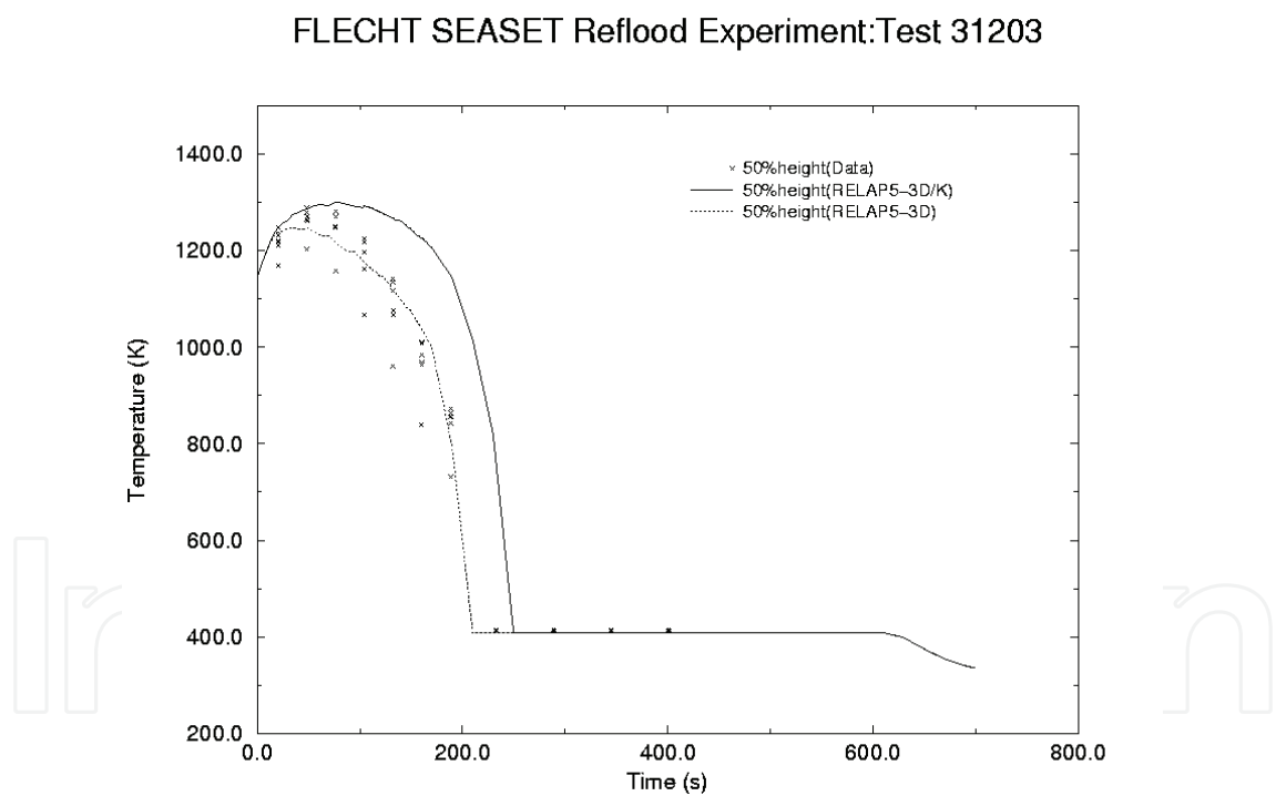
Fig. 11. Comparison of measured and calculated peak cladding temperatures
