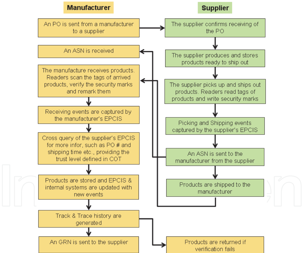
Fig. 8. Logic flow of the OM process enabled by the secure RFID-based track & trace solution
