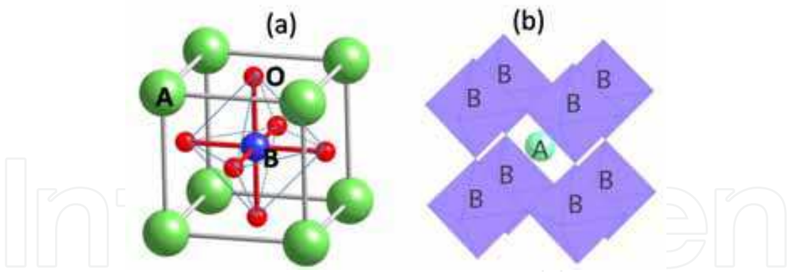
Fig. 1. The structure of an ABO 3 perovskite with the origin centered at (a) the B-site ion and (b) the A-site ion.
