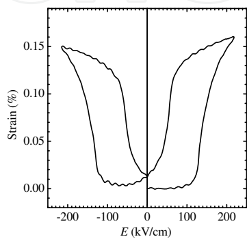
Fig. 5. Strain vs electric field for poly-crystalline AgNbO 3 at room temperature.
