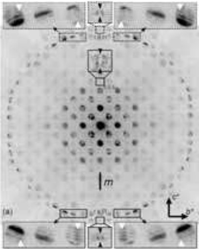
Fig. 6. Convergent-beam electron diffraction (CBED) pattern of \text{AgNbO}_3 taken at the [100] incidence. In contrast to a mirror symmetry perpendicular to the b^* -axis, breaking of mirror symmetry perpendicular to the c^* -axis is seen, indicating that spontaneous polarization is along the c -direction (Taken by R. Sano & K. Tsuda (Sano et al., 2010)).
