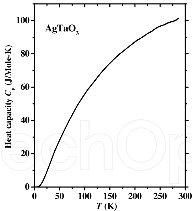
Fig. 25. Heat capacity for AgTaO 3 .
