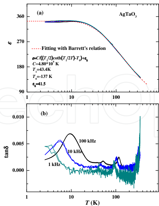
Fig. 24. Temperature dependence of (a) \epsilon together with the fitting to the Barrett's relation indicated by the dashed line and (b) \tan \delta for AgTaO 3 ceramics samples.
