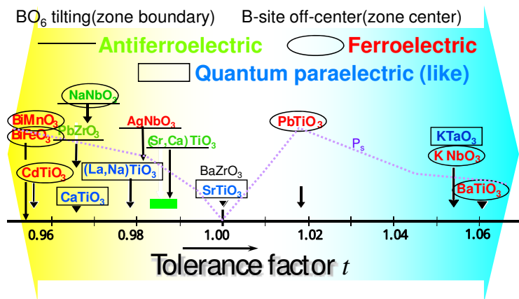
Fig. 2. Tolerance factor of typical dielectric oxides.
