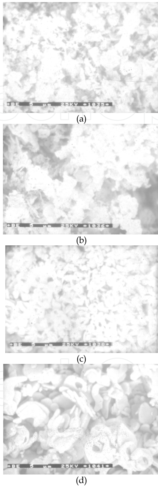
Fig. 10. SEM micrographs of \text{Na}_{0.5}\text{Bi}_{0.5}\text{TiO}_3 powders obtained through route (2) via MSS (NaCl - KCl flux) at different temperatures for 4 h: (a) 800°C; (b) 900°C; (c) 1000°C; (d) 1100°C
