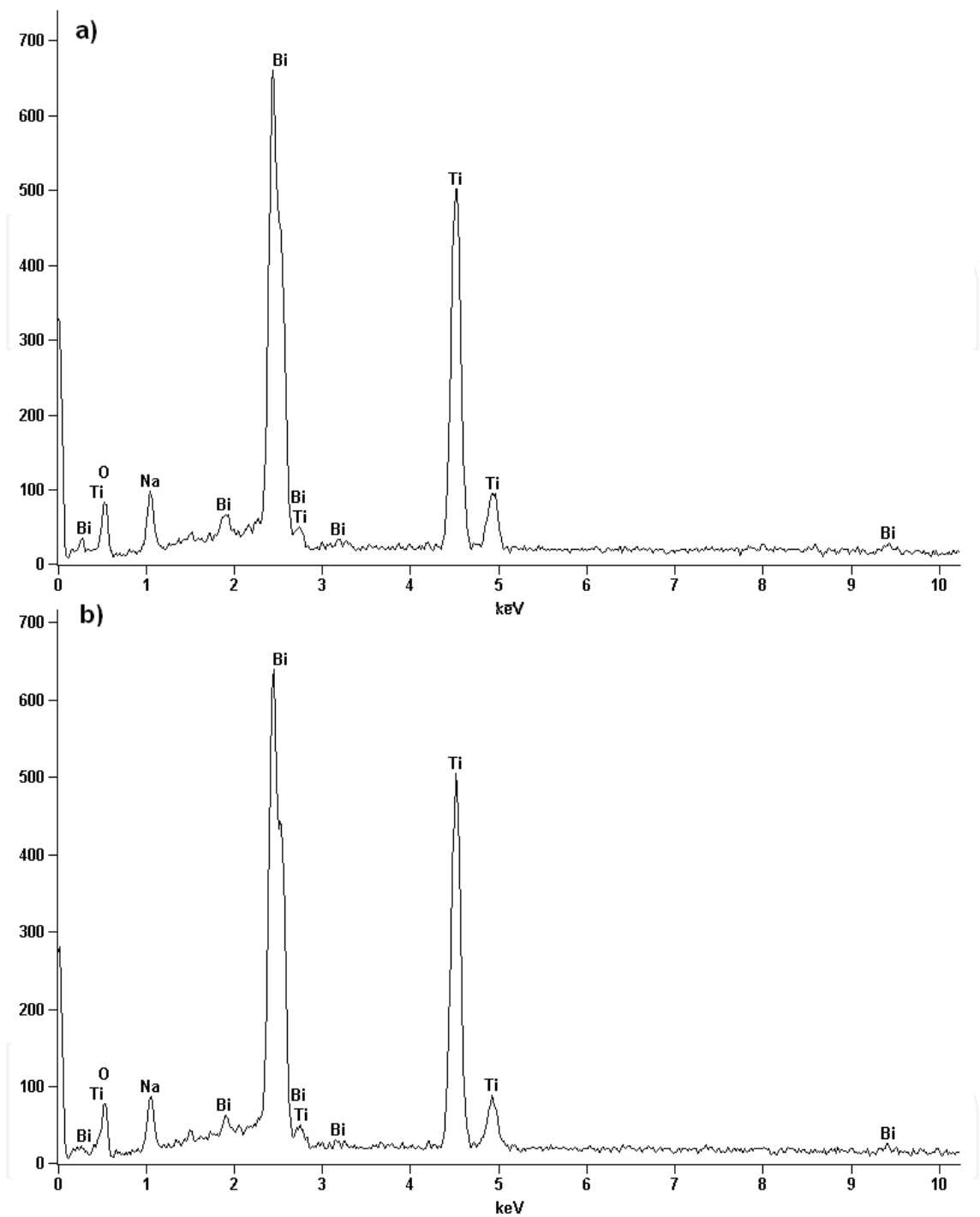
Fig. 12. EDS spectra of of \text{Na}_{0.5}\text{Bi}_{0.5}\text{TiO}_3 powders obtained through route (2) via MSS: (a) NaCl- KCl flux; (b) NaCl flux
