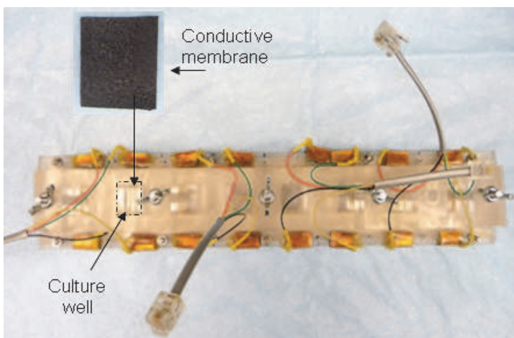
Fig. 3. Home-made multi-well electrical cell culture plate designed for ES
