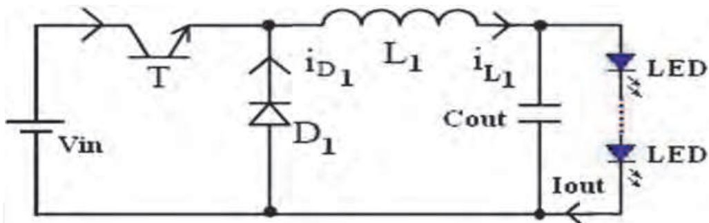
Fig. 3. Buck converter.
