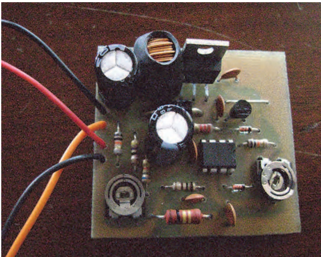
Fig. 8. Buck converter.
