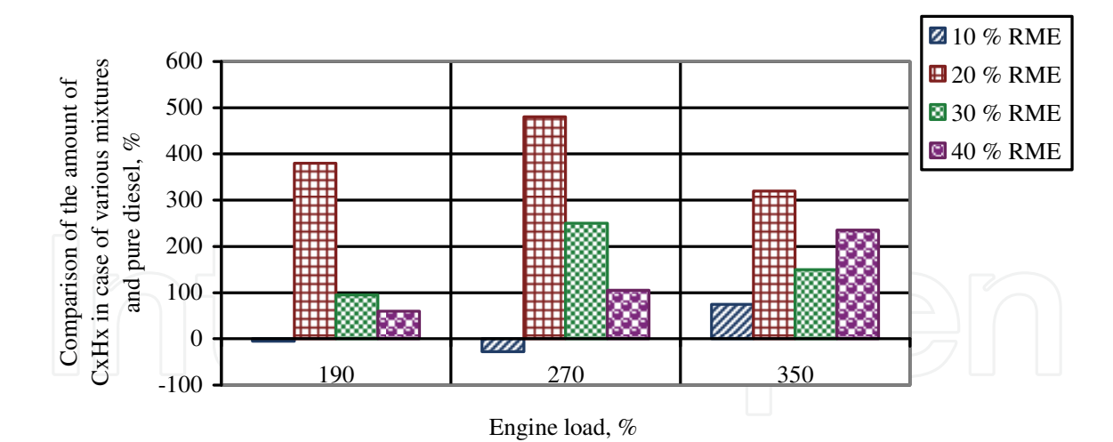
Fig. 15. Percentage comparison of CxHy emission to CxHy emission when using pure diesel
