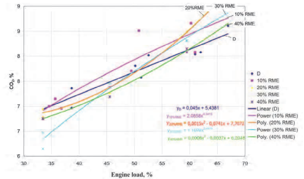
Fig. 11. Dependence of emission of CO 2 on the engine power (% P_{max} ) when using various fuel mixtures
