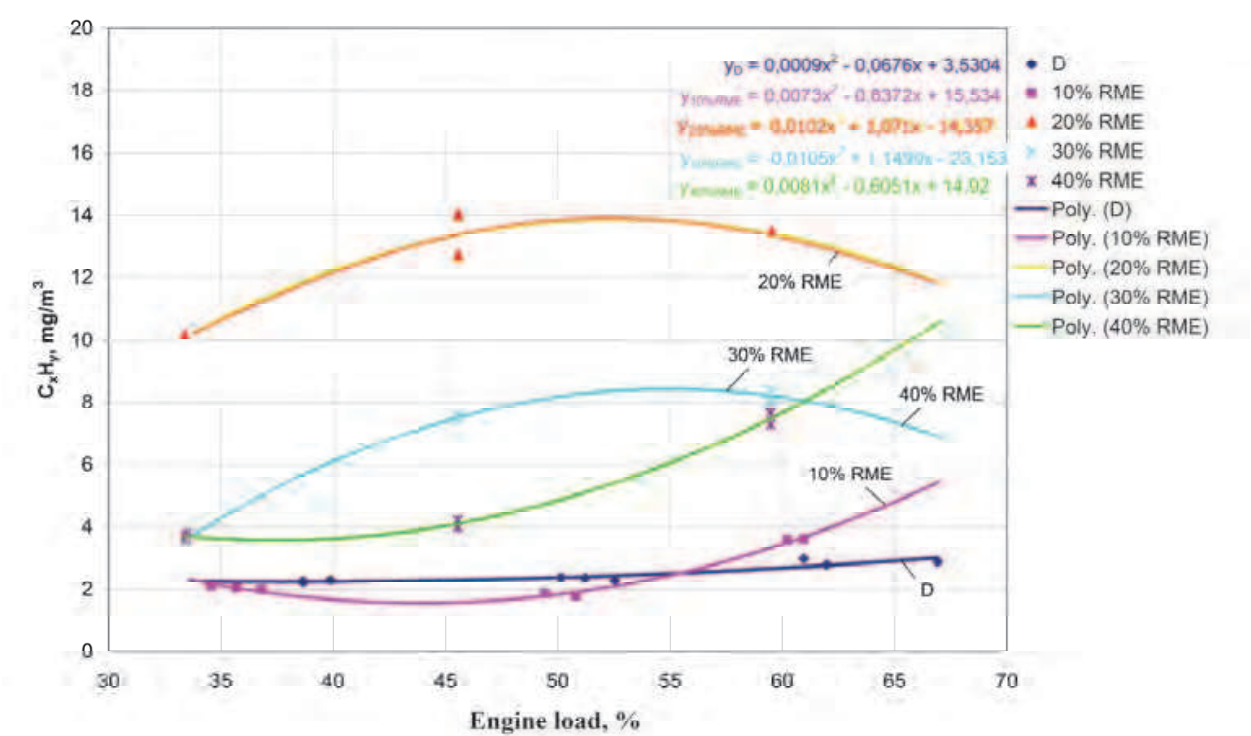
Fig. 14. Dependence of emission of CxHy on the engine power (% P_{max} ) when using various fuel mixtures
