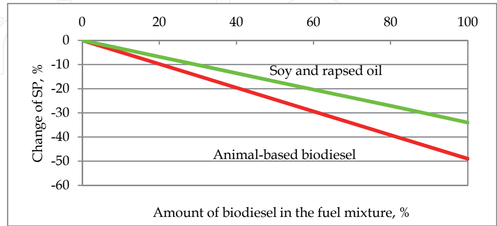
Fig. 4. Dependence of solid particles on the type of biodiesel and the amount thereof in the fuel mixture
