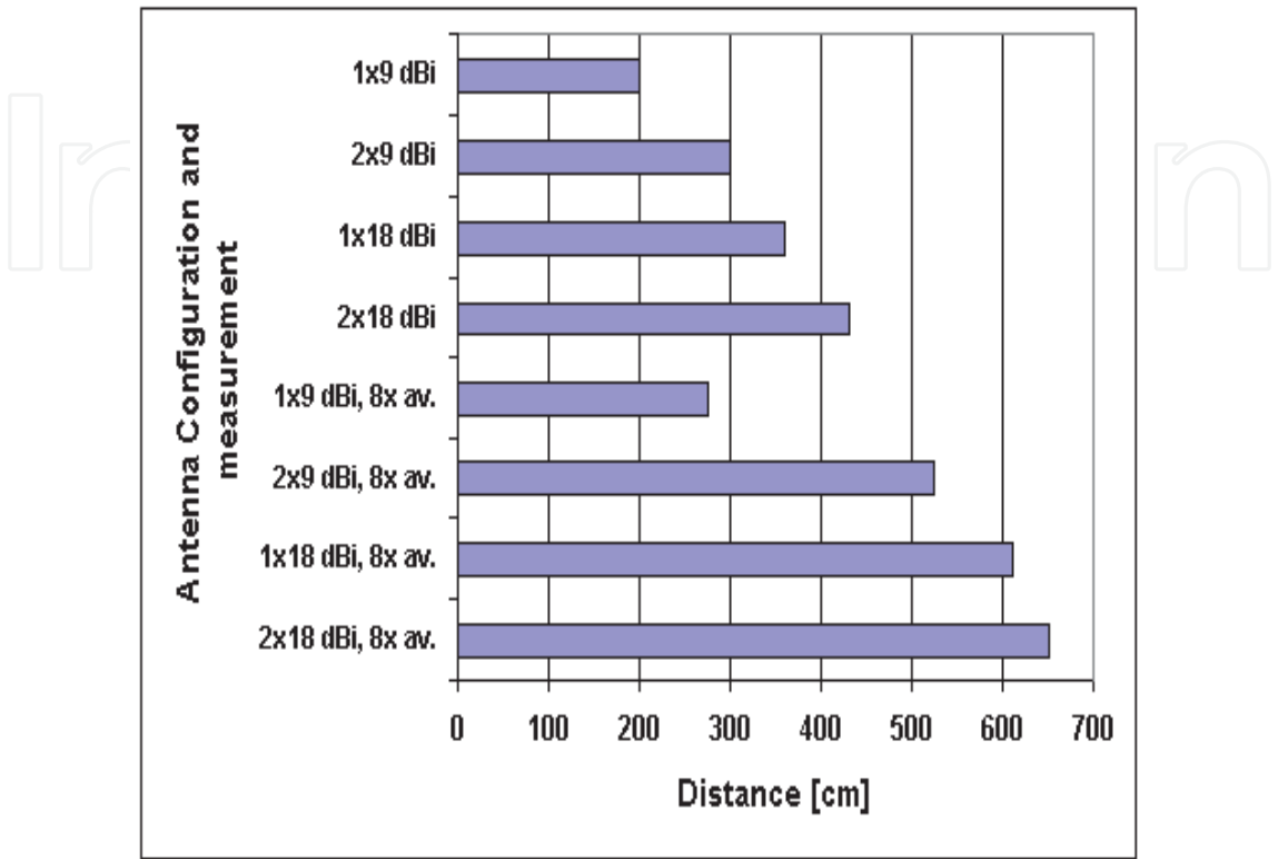
Fig. 10. Read range for various antenna configurations and averaging factors.
