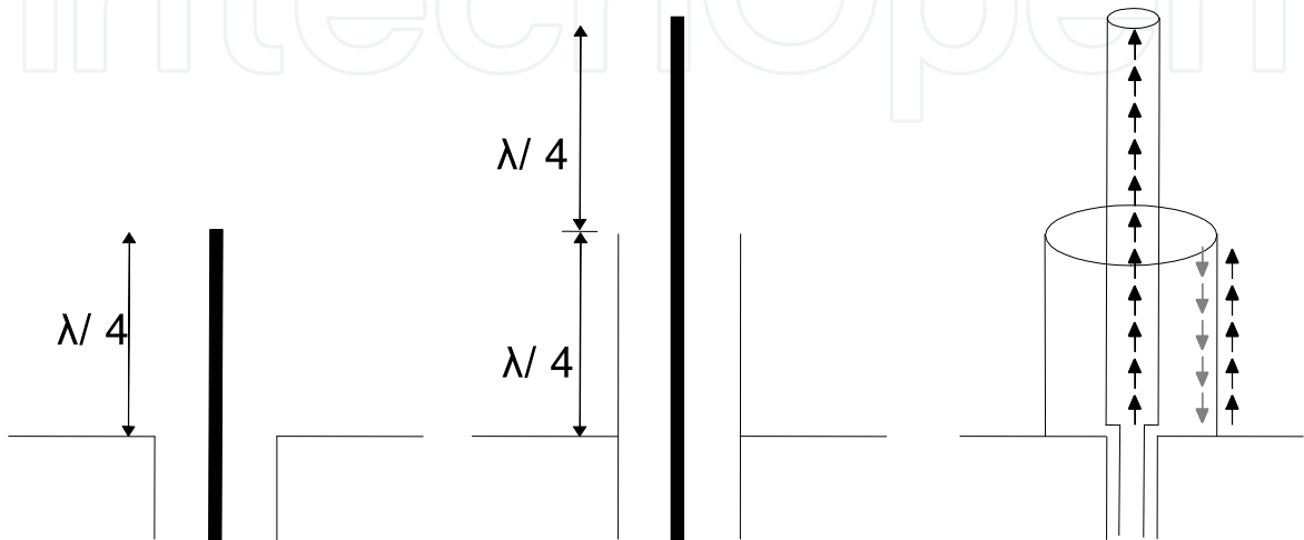
Fig. 1. Traditional monopole over the ground ( left ), Sleeve antenna ( middle ) and 3D-view ( right )
