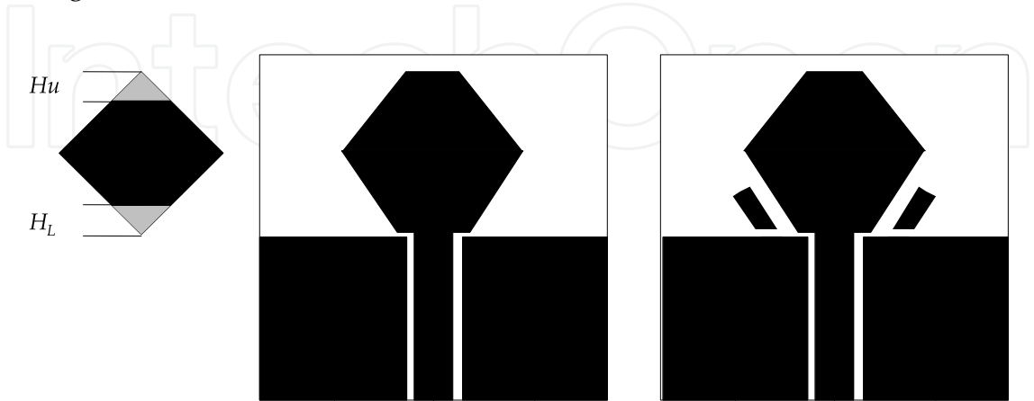
Fig. 12. Schematics of diamond shaped monopole with symmetrical tilted gap sleeves. The tilted gap sleeve has length of 7mm. Sleeve offset from ground and diamond monopole is 0.5mm and 0.75mm
