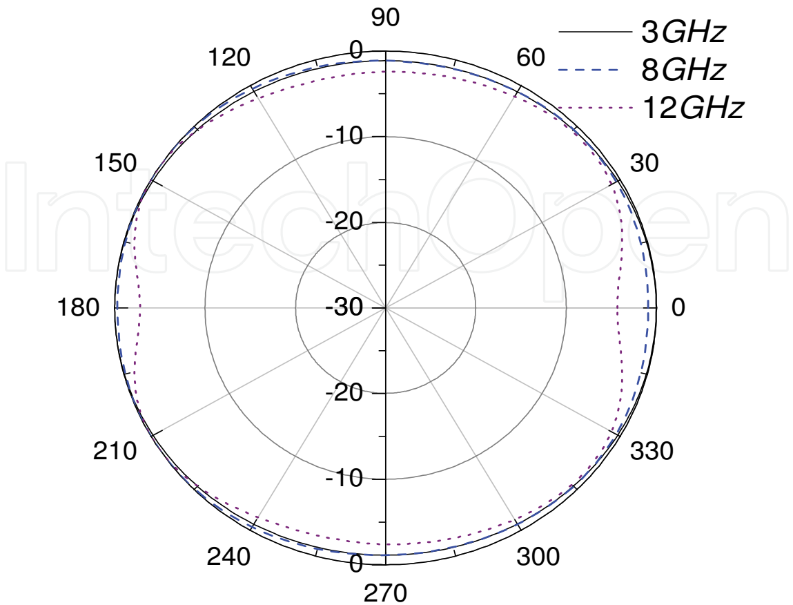
Fig. 15. Azimuth radiating pattern (H-plane) of the proposed diamond shaped coplanar antenna with tilted shapes normalized to 0dB.
