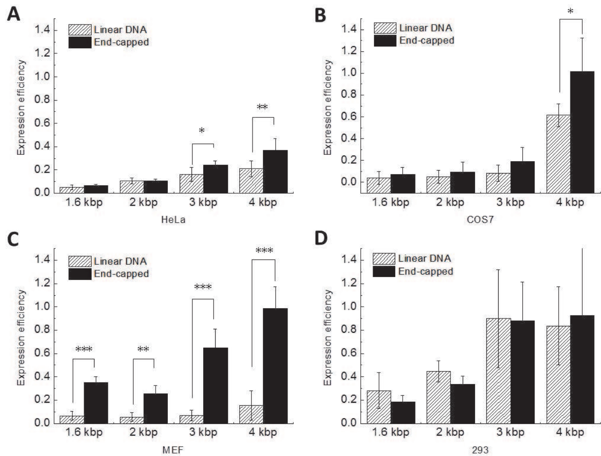
Fig. 11. Effect of DNA protection against exonucleases on expression efficiency with a cationic lipid. (A) HeLa, (B) COS7, (C) MEF and (D) 293 cells were transfected with 1 \mu g of uncapped or capped linear DNA per well. Complexes were formed with LipofectAmine 2000 reagent. Expression efficiency (E/Ep) is expressed as the mean \pm S.D. of 4–5 different experiments. To normalize the values from each individual experiment, the expression rate of DNA was divided by the rate using the pEGFP-C1 plasmid. *, P < 0.05 ; **, P < 0.01 ; ***, P < 0.001 (Student's t test). Striped bars, uncapped linear DNA; brack bars, end-capped DNA.
