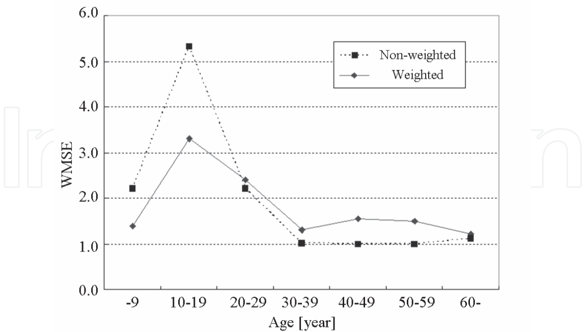
Fig. 4. WMSE for each age-group.
