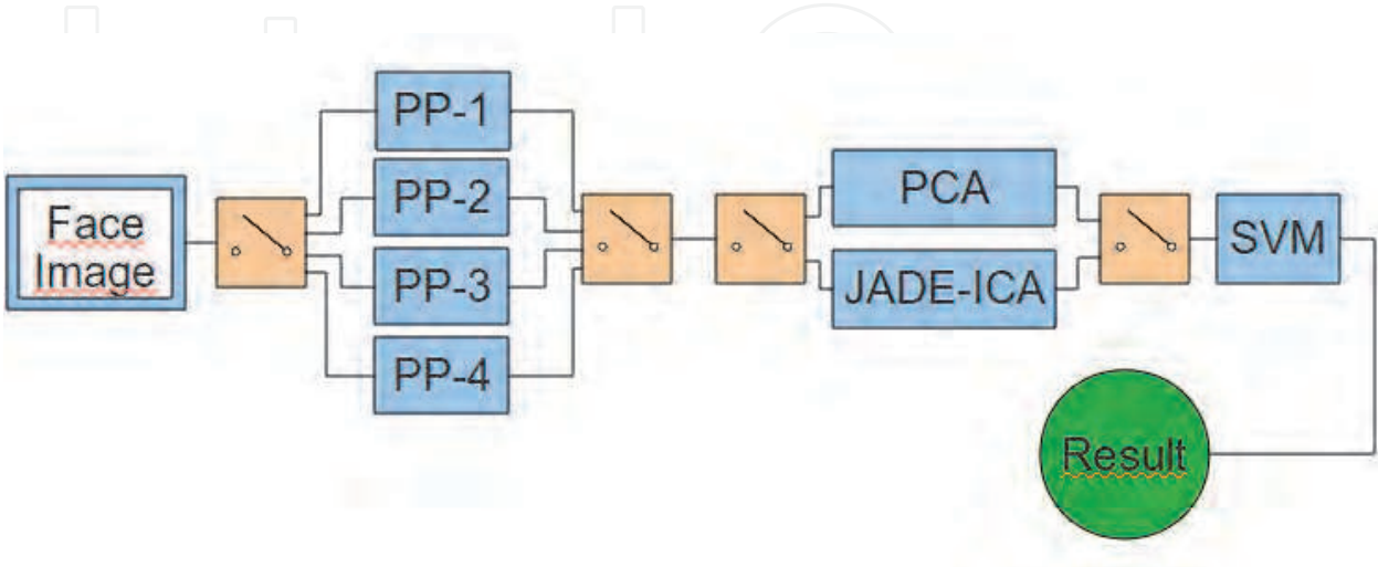
Fig. 6. Block diagram of the implemented system
