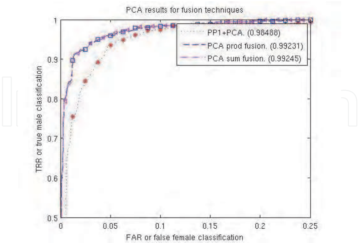
Fig. 10. Curves obtained for each score fusion of each preprocessing technique and PCA. In legend numbers represents the area under the curve.
