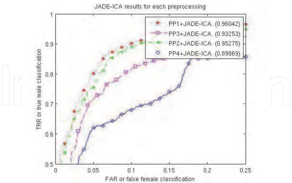
Fig. 9. Curves obtained for each preprocessing and JADE-ICA. In legend numbers represents the area under the curve.
