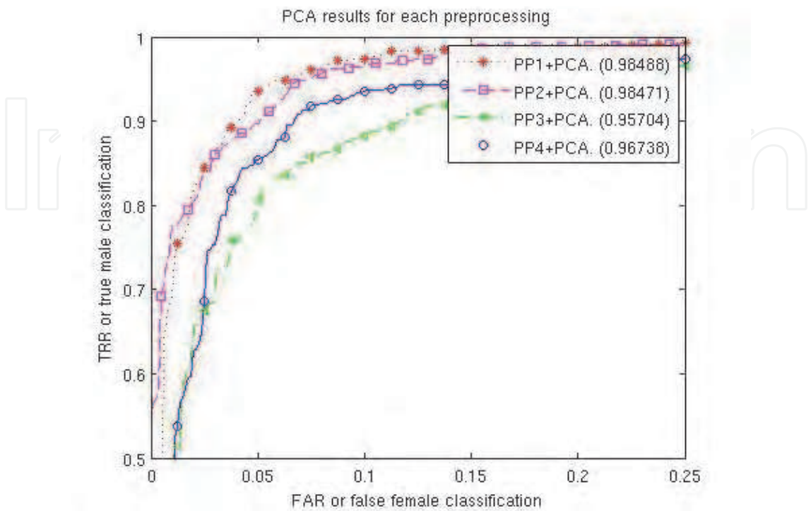
Fig. 8. Curves obtained for each preprocessing and PCA. In legend numbers represents the area under the curve.
