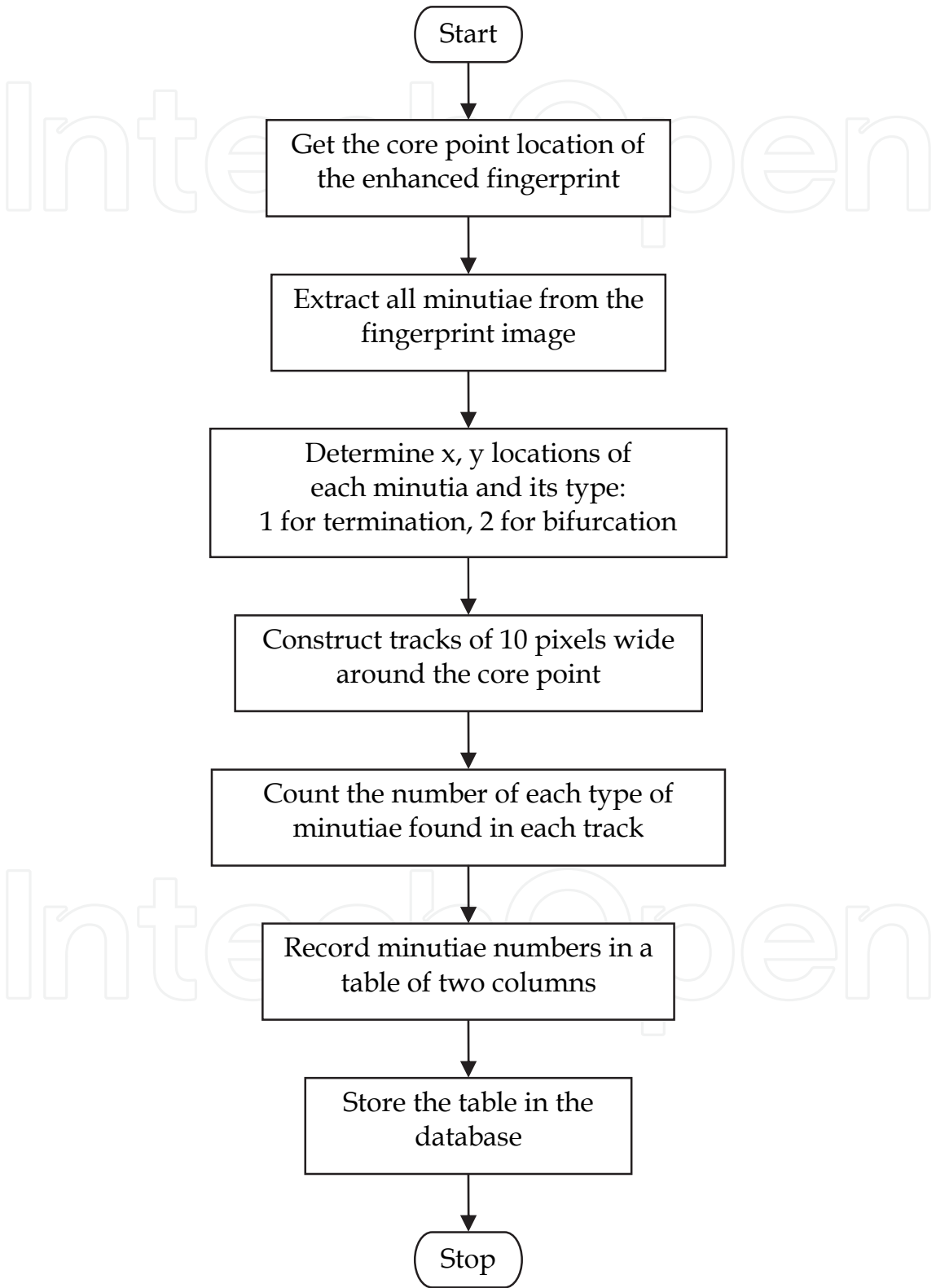
Fig. 2. Flowchart of the enrolment phase of the proposed matching algorithm.
