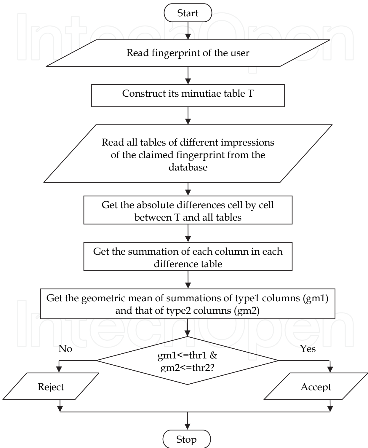
Fig. 3. Flowchart of the proposed verification phase.
