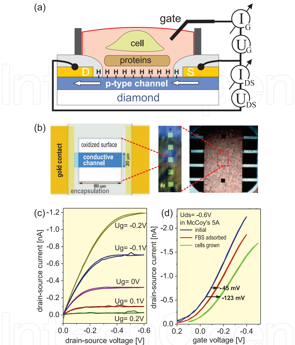
Fig. 10. (a) Diagram of a solution-gate field-effect transistor (SG-FET) based on the surface conductivity of hydrogen-terminated diamond. The insulation of the SG-FET gate is ensured merely by the hydrogen termination of the diamond channel surface. Thus, proteins and cells react directly with the surface of diamond. (b) Top-view: hydrogen-terminated conductive microscopic channel is surrounded by insulating oxygen-terminated areas and the active area is determined by the hole in the insulating layer. A chip contains several such areas, as is demonstrated in the optical image of the whole chip ( 10 \times 10 \text{ mm}^2 with 5 transistors) on the right. (c) Output characteristics of SG-FET transistor from nanocrystalline diamond in McCoy's 5A solution with gate potential between -0.2 and 0.2 \text{ V} . (d) Transfer characteristics of a transistor in McCoy's 5A solution at the beginning of the experiment (blue), after the adsorption of proteins from FBS (red) and after 48h cell cultivation (green)
