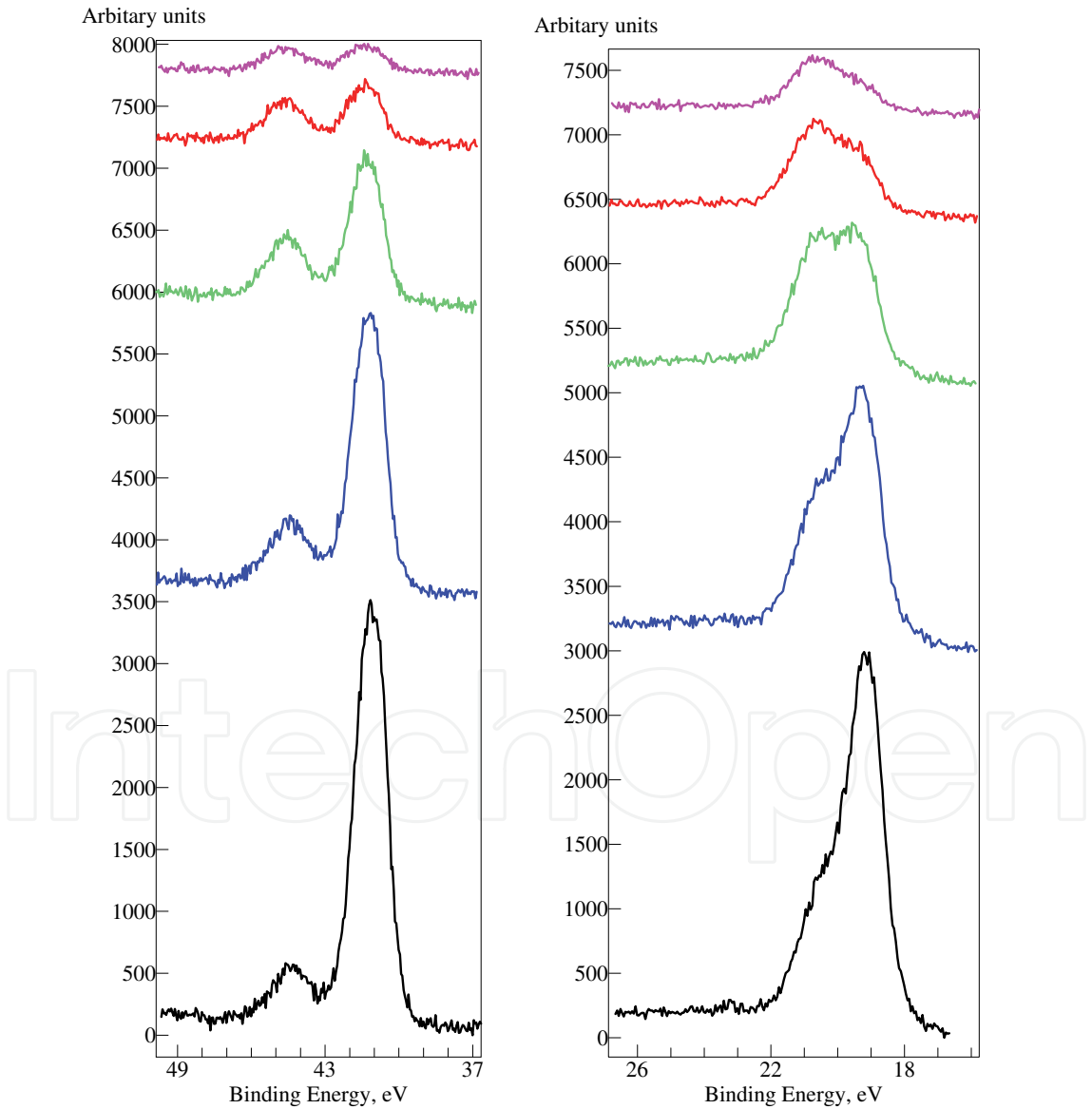
Fig. 6. ARXPS spectra of As 3d (left) and Ga 3d (right) for TOA angles:90°-black, 50° blue, 30° -green, 20°-red, 15°-pink
