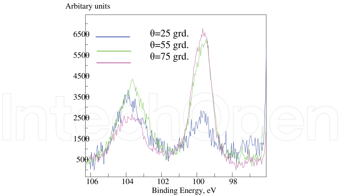
Fig. 4. SiO 2 /Si native oxides XPS proportional spectra
