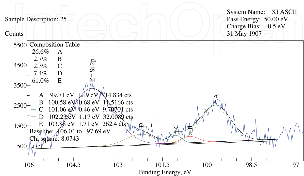
Fig. 5. XPS spectra for Si (oxidized) S0 sample at TOA=25 0
