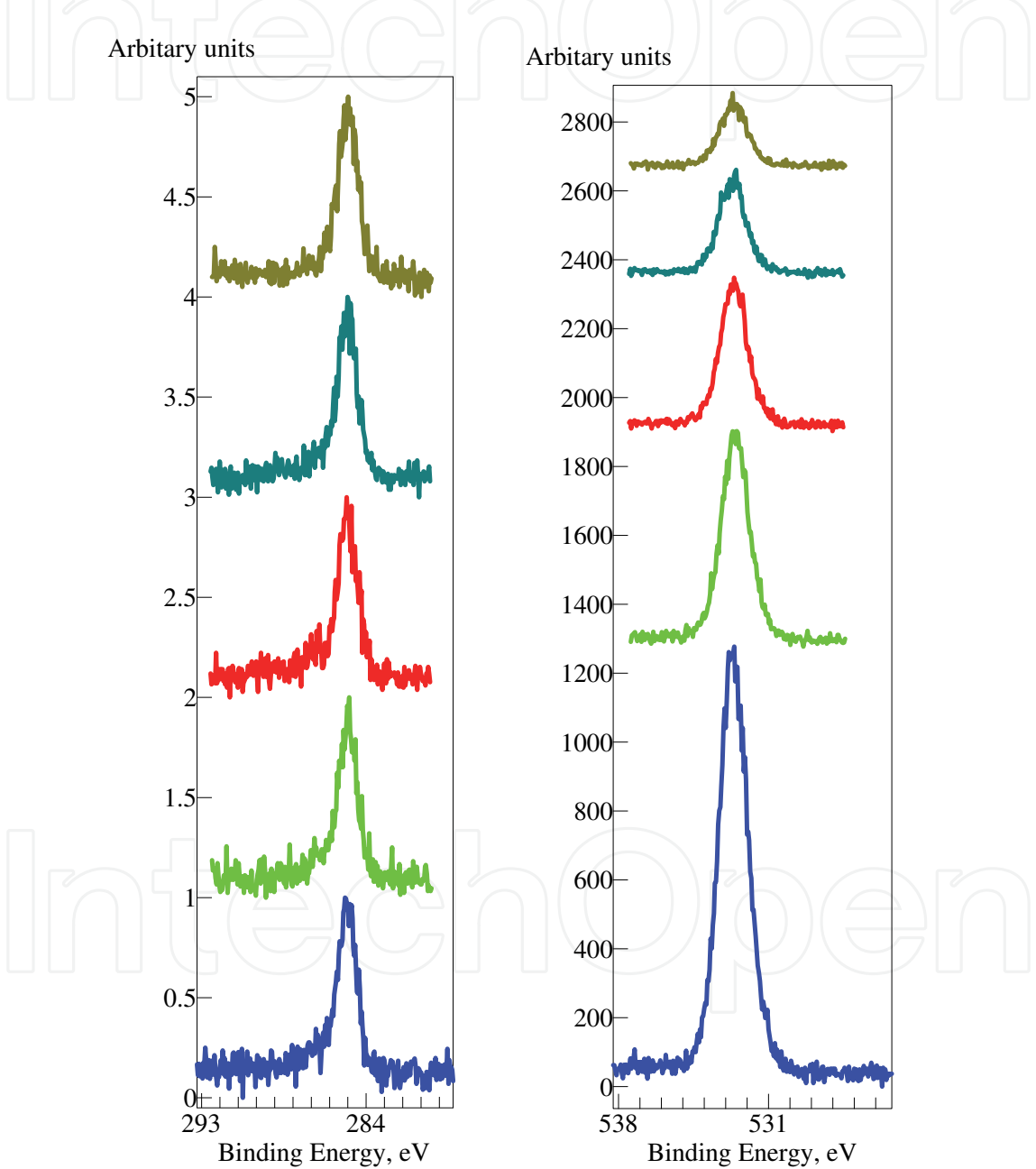
Fig. 9. ARXPS spectra for C1s(left) and O1s (right) at TOA: 90°(blue), 50°(green),30°(red), 20°(turquoise), 15°(olive)
