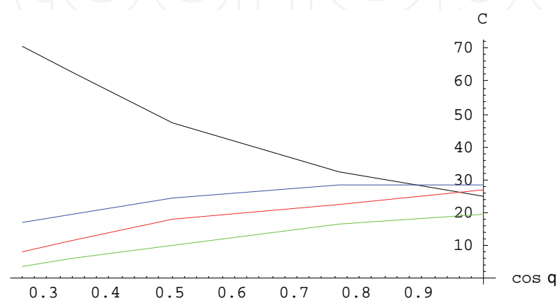
Fig. 7. Relative variation of concentration for C-black, O-blue, As-green and Ga-red as a function of analysis angle (q) (TOA=90 0 -q)
