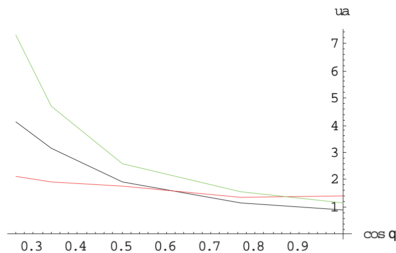
Fig. 8. Variation of different concentration ratios for C c /C 0 -black, C Ga /C As -red, C c +C 0 /C Ga +C As -green as a function of analysis angle (q) (TOA=90-q)
