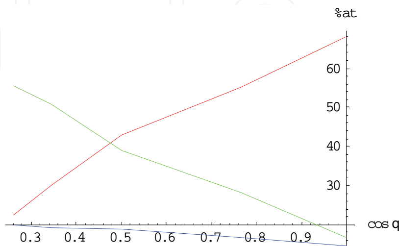
Fig. 13. (a) Concentration variation of Si 0 (red), SiO 2 (green) and SiO x (blue) at TOA(90°-q) for the ARXPS signal of Si 2p
