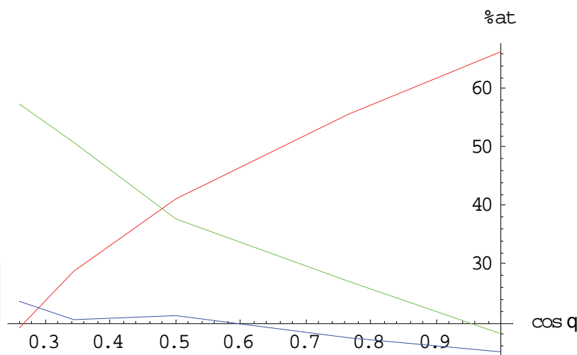
Fig. 13. (b) Concentration variation of Si 0 (red), SiO 2 (green) and SiO x (blue) at TOA (90°-q) for the ARXPS signal of Si 2s
