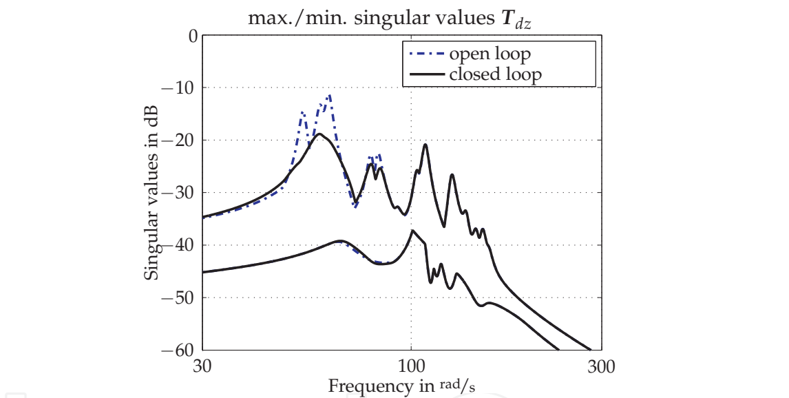
Fig. 21. Reduction of rail car disturbance transfer singular values with collocated \mathcal{H}_2 control collocated acceleration sensors (see Section 3.1.3) did not yield satisfactory performance. The singular value plot shows only marginal magnitude reduction (Figure 12), and also a time-domain analysis of the performance signals z_1 and z_6 (see Figure 13) shows no significant improvement. According to Table 2, the reduction of the filtered performance vector is approximately 8%. However, at \omega \approx 1500 \text{ rad/s} one of the frequency response modes approaches the imaginary axis (Fig. 14 and Fig. 15). Even though the simulated closed loop remains stable, this spillover is critical for operation at an uncertain real plant which possesses unknown high-frequency dynamics. Considering the LQG design for non-collocated strain sensors in Section 3.1.2, the controller significantly improves the vibrational behaviour. The performance vector is reduced by 23% (Table 1) and a significant reduction is apparent for the time-domain evaluation in Fig. 9. The maximum singular values of the first three eigenmodes are reduced (e.g. third eigenmode
