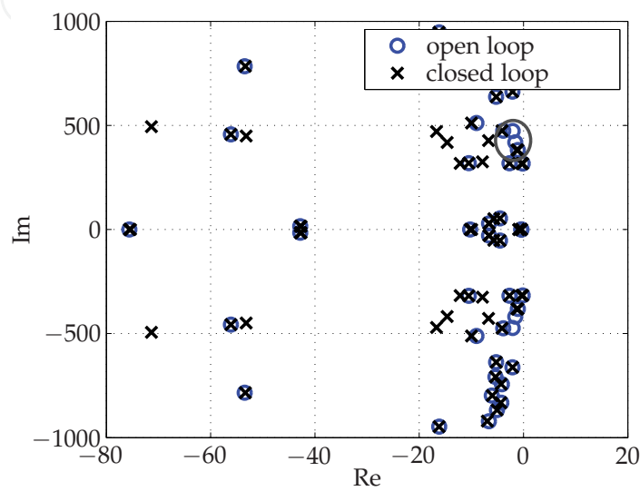
Fig. 29. Pole plot with/without LQG controller
