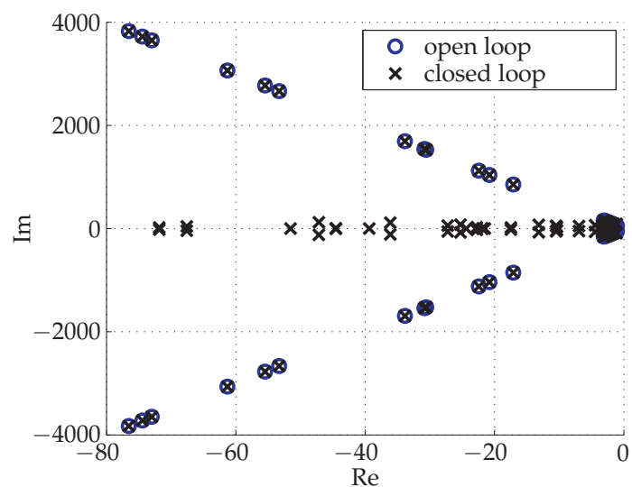
Fig. 19. Rail car model open-loop and non-collocated \mathcal{H}_2 closed-loop pole locations by (3)) to the performance vector z , the time-domain response of two selected performance variables z_1 and z_6 , and two pole location plots (overview and zoomed) for the open- and the closed-loop results.
