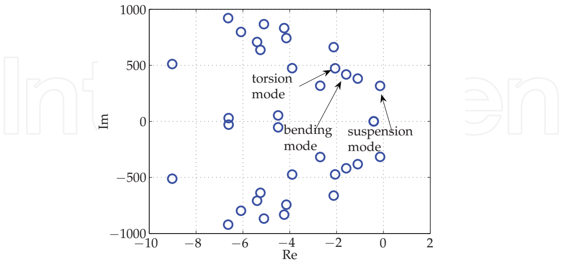
Fig. 27. Pole plot of the identified scaled metro car body (zoomed)
