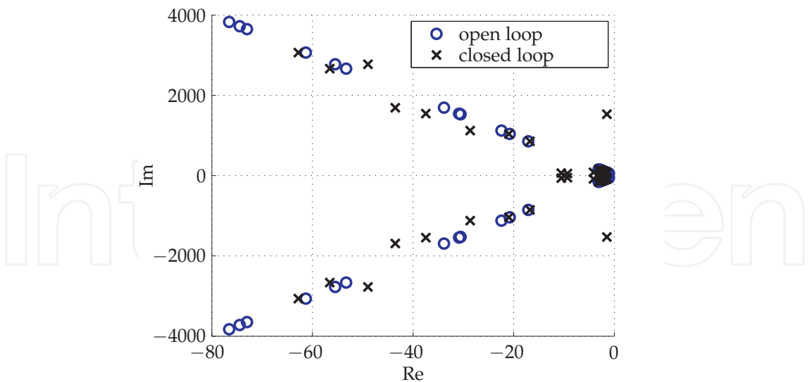
Fig. 14. Rail car model open-loop and collocated LQG closed-loop pole locations
