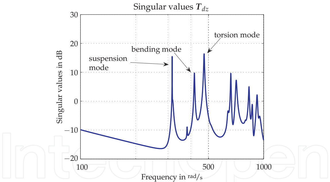
Fig. 28. Singular values of the identified scaled metro car body
