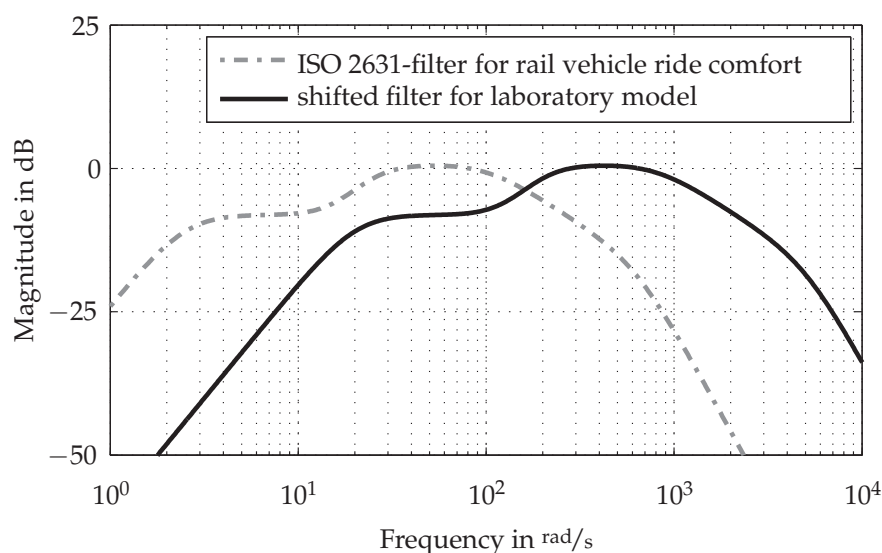
Fig. 5. Filter function according to ISO 2631 (yaw axis)
