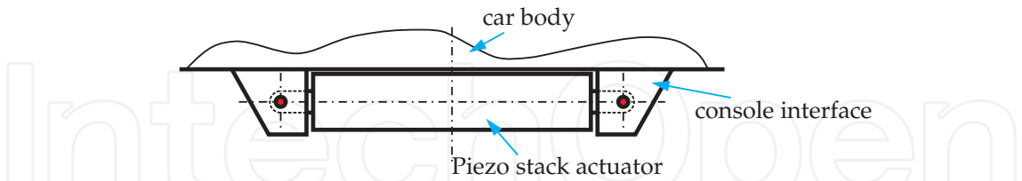
Fig. 3. Actuator mounted in a console to introduce torques into the attached flexible structure (rail car body)
