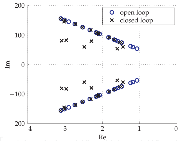
Fig. 11. Rail car model open-loop and non-collocated LQG closed-loop pole locations (zoomed)
