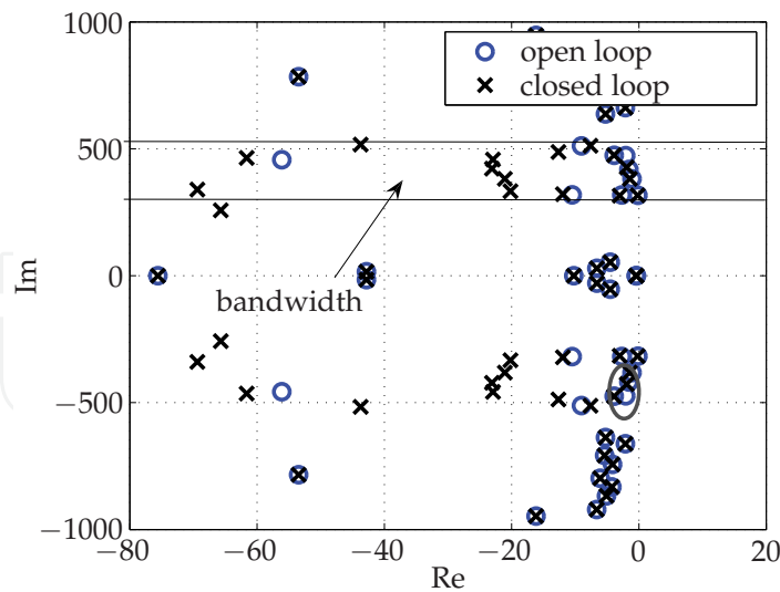
Fig. 31. Pole plot with/without \mathcal{H}_2 controller
