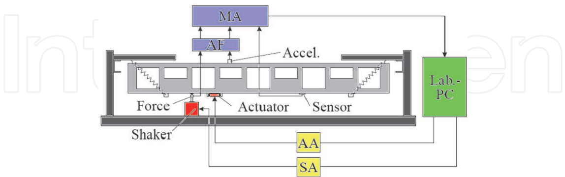
Fig. 26. Basic sketch of the scaled metro car body with actuators, sensors, and performance variables
