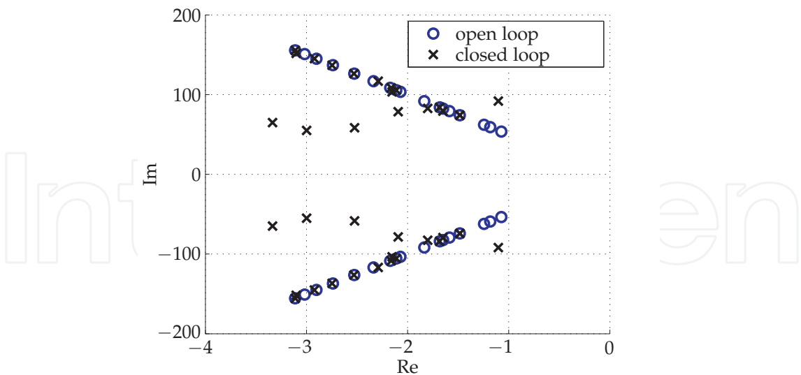
Fig. 20. Rail car model open-loop and non-collocated \mathcal{H}_2 closed-loop pole locations (zoomed)
