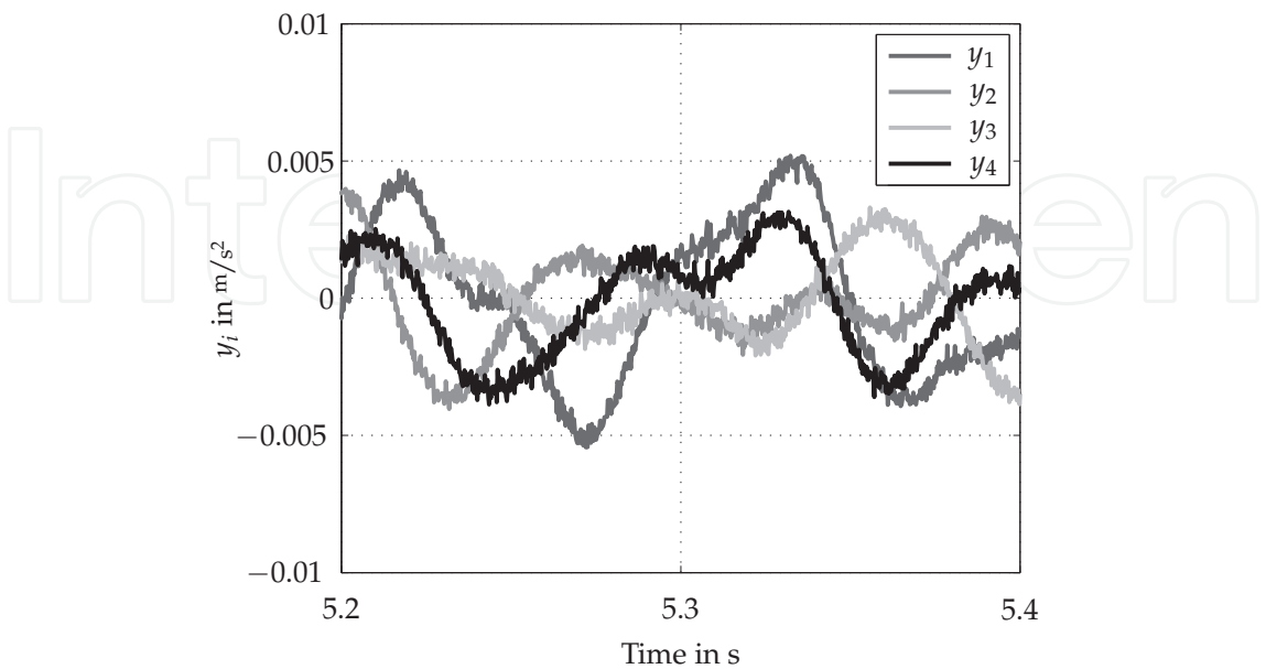
Fig. 4. Measured acceleration signals of the sensors showing a signal-to-noise ratio SNR = 10
