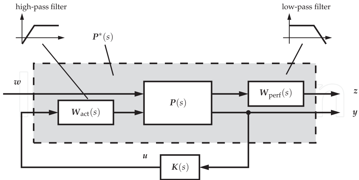
Fig. 16. Closed-loop system P(s) with controller K(s) and actuator and performance weighting functions W_{\text{act}}(s) and W_{\text{perf}}(s)
