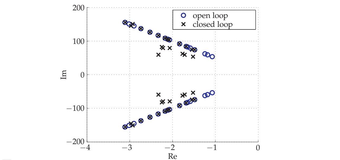
Fig. 15. Rail car model open-loop and collocated LQG closed-loop pole locations (zoomed)
