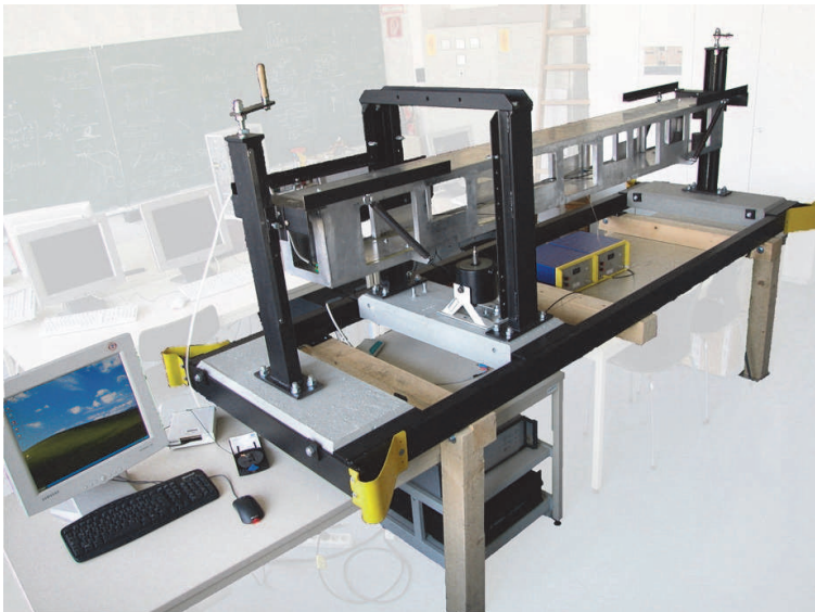
Fig. 25. Scaled metro car body
