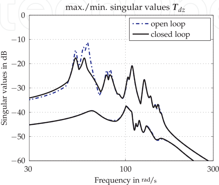
Fig. 8. Reduction of rail car disturbance transfer singular values with non-collocated LQG control
