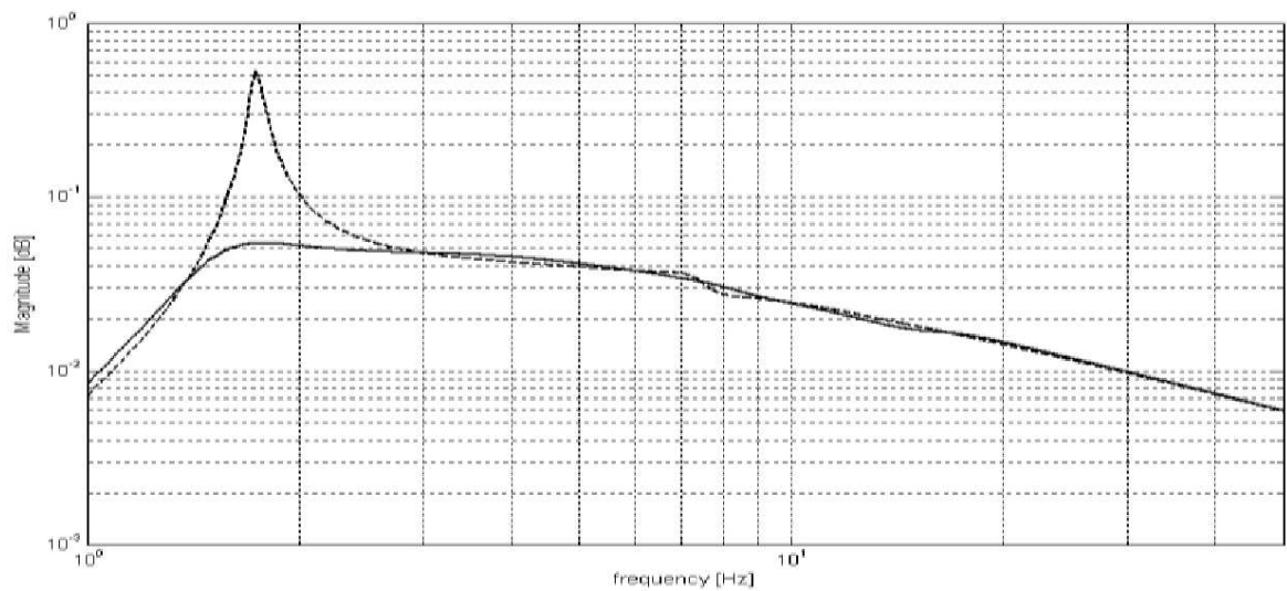
Fig. 19. Vibration damping action. Transfer function from a force applied on the stage to the velocity measured on the stage ( \dot{q}_S/F_{STAGE} ) . Numerical response. Solid line: closed-loop; Dashed line: Open-loop.
