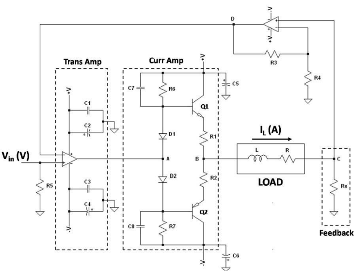
Fig. 12. Power electronic based on a trans-conductance amplifier.
