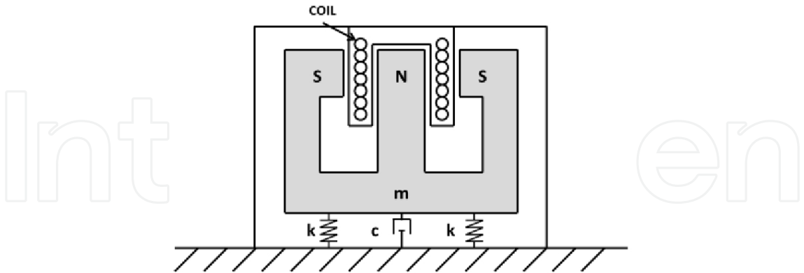
Fig. 8. Geophone reverse configuration scheme.
