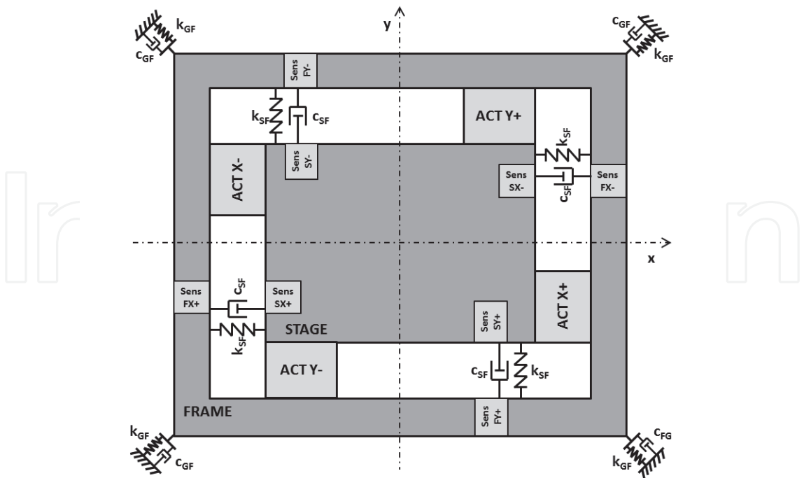
Fig. 2. XY plane view of the system. Frame-stage spring ( k_{FS}, c_{FS} ), electromagnetic actuator (ACT), velocity sensor (Sens.), Frame-Ground spring ( k_{FG}, c_{FG} ).
