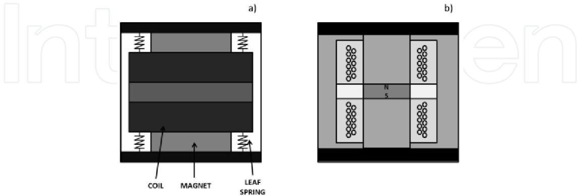
Fig. 7. Geophone active configuration scheme. a) Coil and springs installation. b) Cross section.
