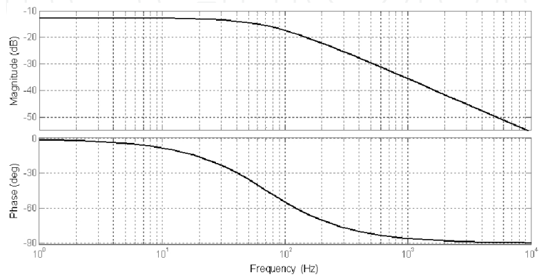
Fig. 6. Actuator trans-conductance transfer function (magnitude and phase).
