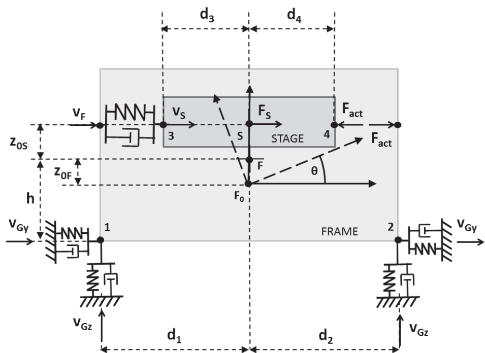
Fig. 15. YZ plane 4dof model scheme – input and output. Using the Lagrange formulation is possible to write the equations of motion in the form:
