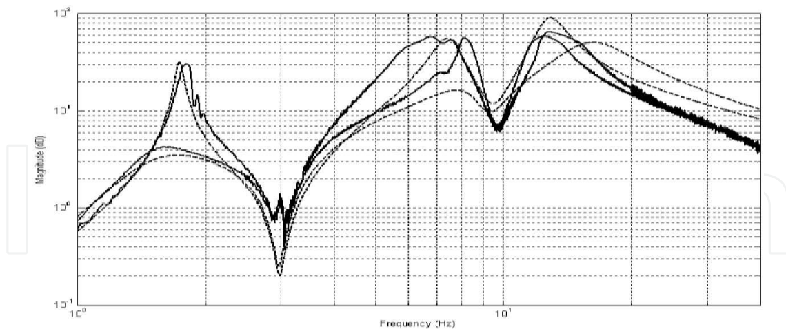
Fig. 17. Vibration damping action. Transfer function from the actuator force to the difference of frame and stage velocities ((\dot{q}_S - \dot{q}_F)/F_{ACT}) . Open-loop vs Closed-loop. Solid line: experimental; Dashed line: numerical.
