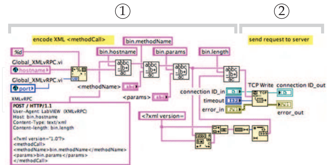
Fig. 6. Block diagram of the the XMLvRPC_WriteRequest.vi.
