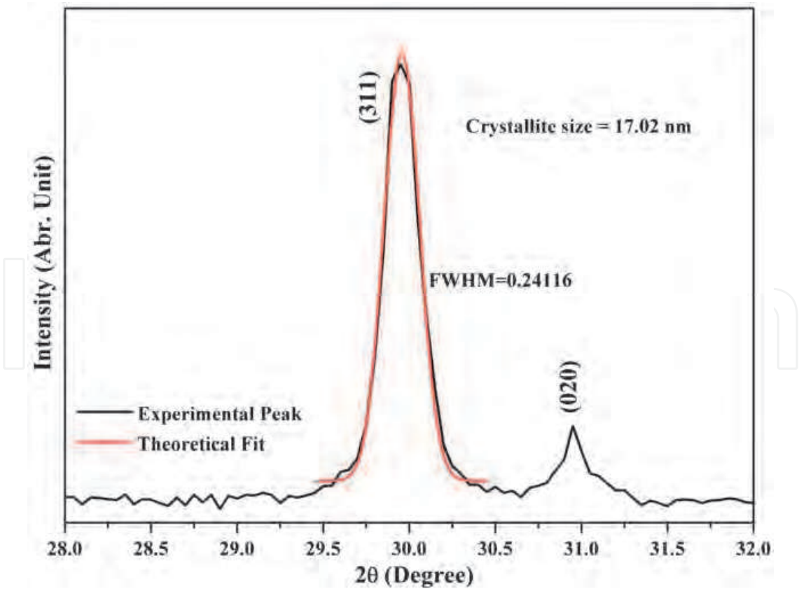
Fig. 4. Maximum intense peak in XRD pattern of nanostructured ZN ceramics with theoretical Gaussian Fit
