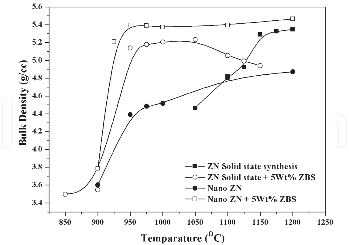
Fig. 8. Variation of the bulk density of ZN ceramics and ZN-glass composites with different temperature
