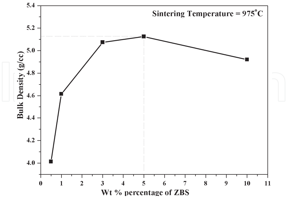
Fig. 7. Variation of bulk density of ZN ceramics (solid state synthesis) with different wt% of ZBS glass
