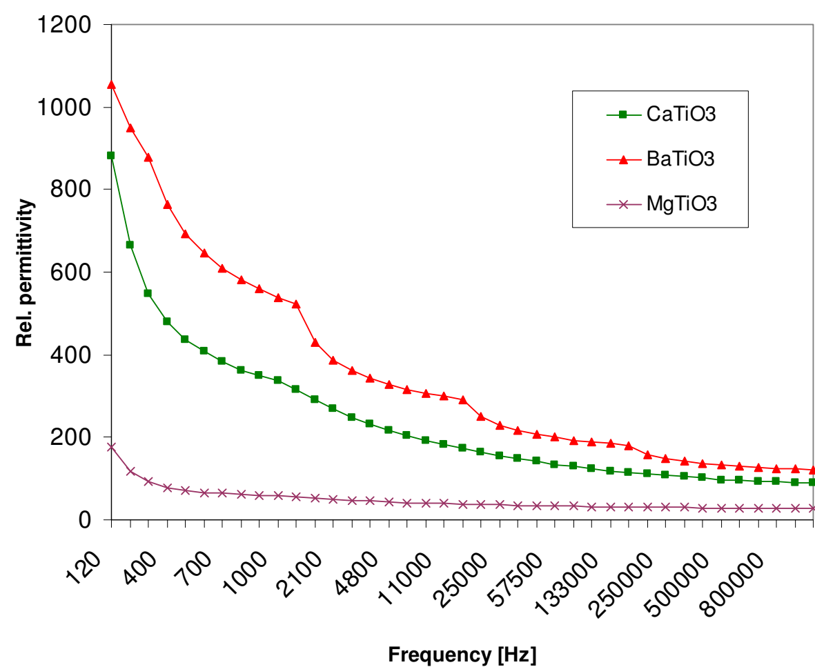
Fig. 14. Frequency dependence of the relative permittivity of plasma sprayed BaTiO 3 , CaTiO 3 , and MgTiO 3 at room temperature
