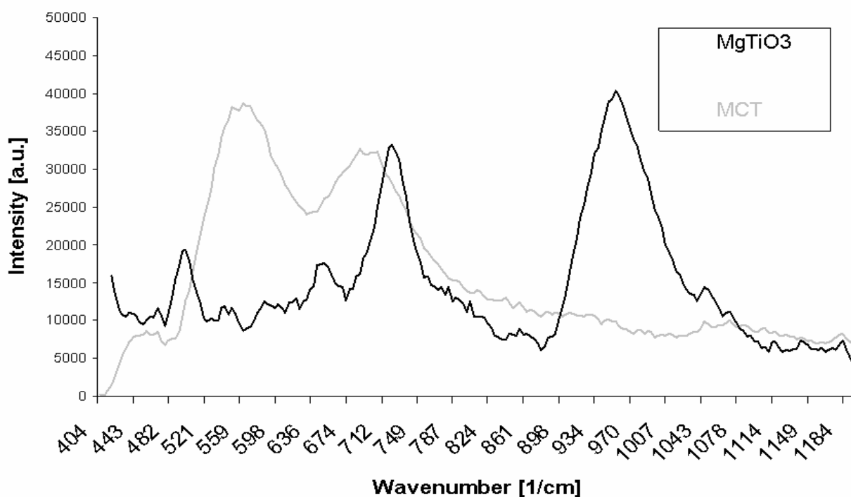
Fig. 3. Raman spectrum of MCT
