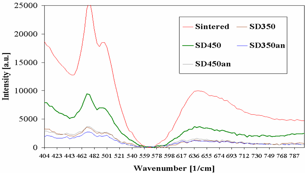
Fig. 1. Raman spectrum of \text{CaTiO}_3
