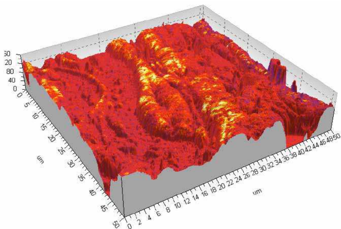
Fig. 20. Superposition of the AFM contact mode image and SMM image - BaTiO 3 cross section. Hard and high-permittivity Ti-rich lamellae are yellow
