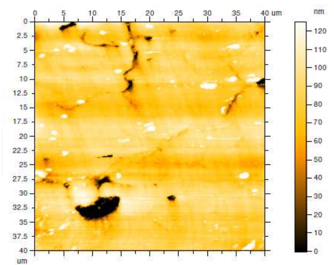
Fig. 17. AFM contact mode image of BaTiO 3 (in plane orientation). Roughness representation: peaks are lighter and valleys darker (black color represents pores)
