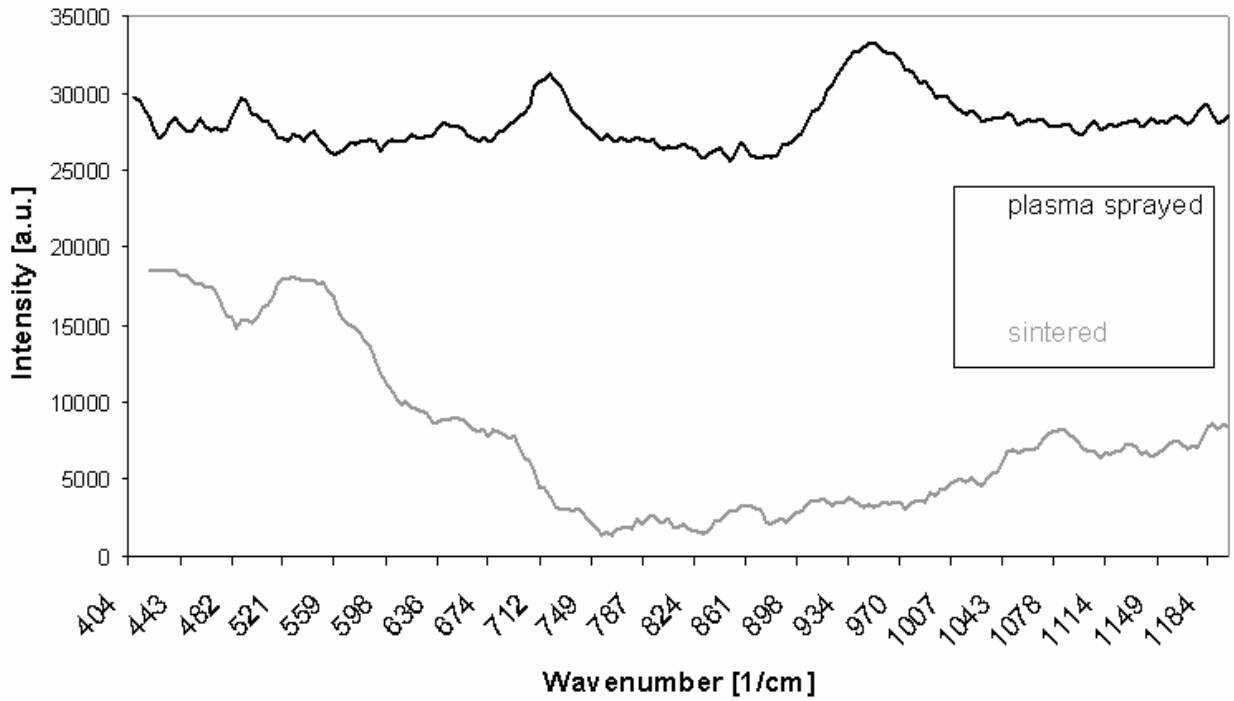
Fig. 2. Raman spectrum of \text{MgTiO}_3
