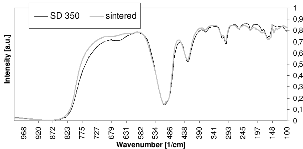
Fig. 7. Infrared spectrum of CaTiO 3
