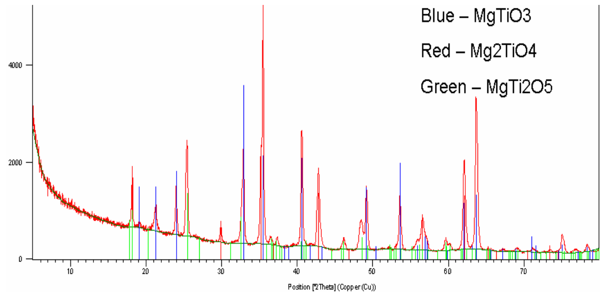
Fig. 8. XRD pattern of plasma sprayed MgTiO 3
