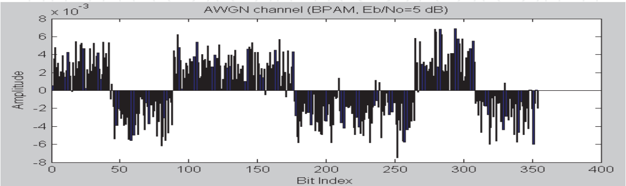
Fig. 4.9. AWGN channel output (BPAM), where Eb/No=5 dB.
