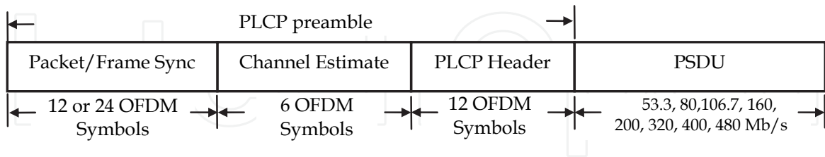
Fig. 2. PPDU structure
