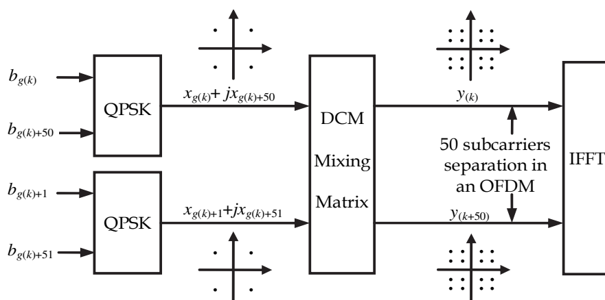
Fig. 13. DCM mapping process
