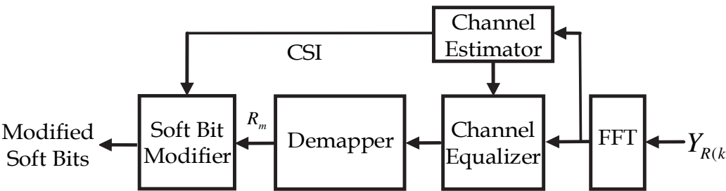
Fig. 16. Demodulation exploiting CSI
