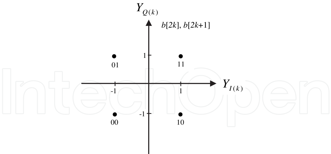
Fig. 5. QPSK constellation mapping
