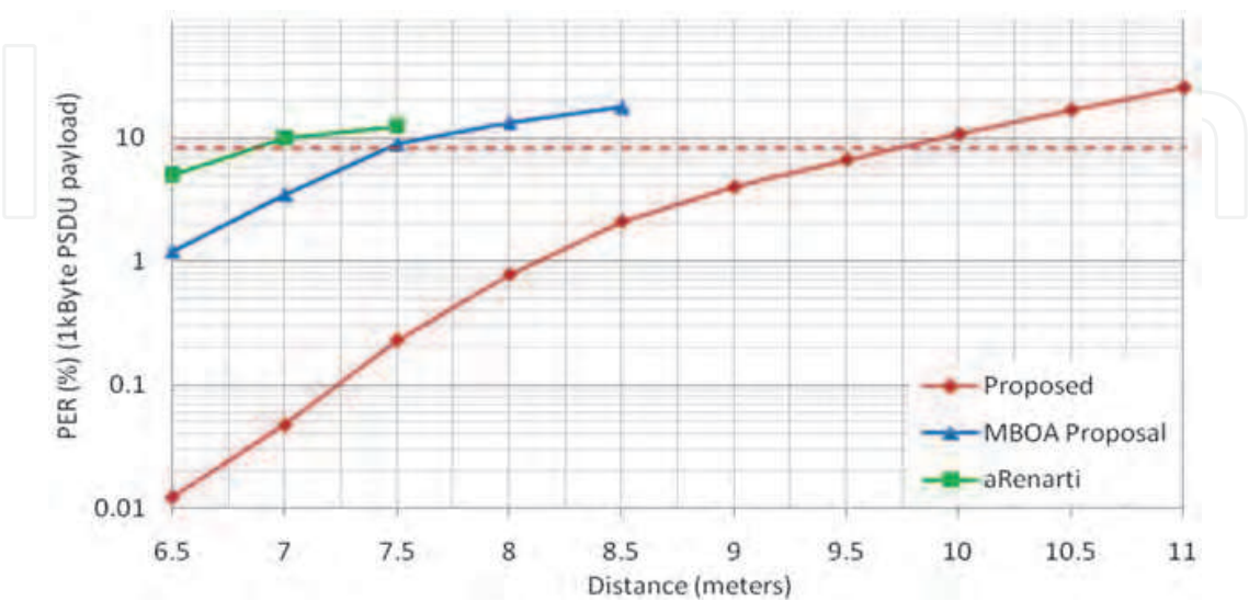
Fig. 11. Performance comparison for 200 Mb/s mode in CM1
