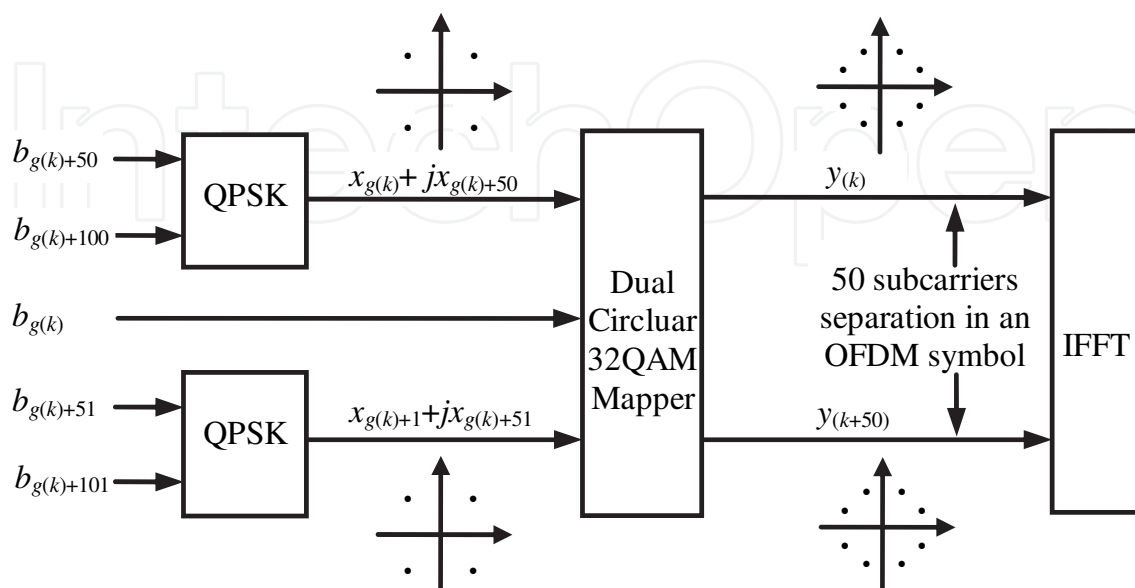
Fig. 21. DC 32-QAM mapping process
