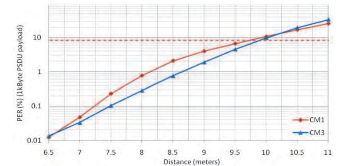
Fig. 10. System performance for 200 Mb/s mode in CM1 and CM3
