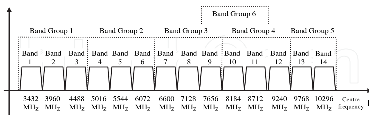
Fig. 1. Band group allocation (ECMA-International, 2008)
