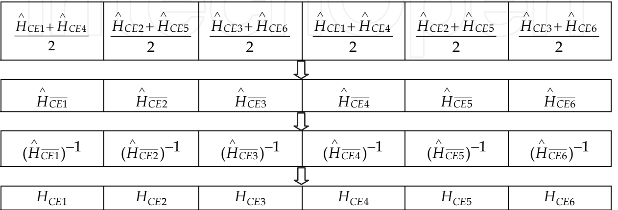
Fig. 14. Averaged and inversed channel estimation sequences for TFC=1, BG=1
