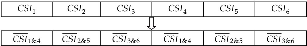
Fig. 15. Averaged CSI blocks allocation for TFC=1, BG=1
