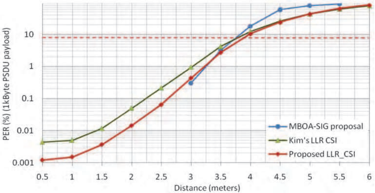
Fig. 18. Performance comparison for 480 Mb/s mode in CM1
