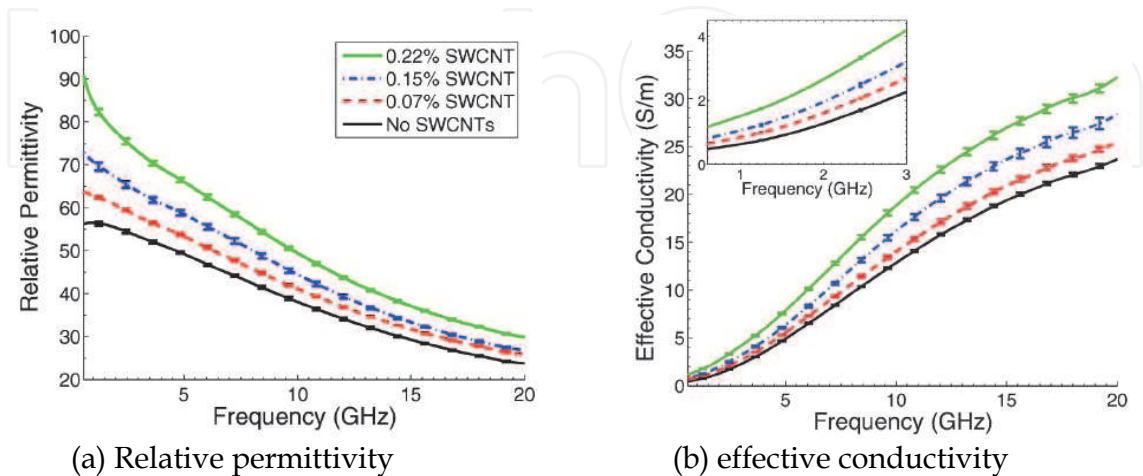
Fig. 14. Electrical properties of tissue-mimicking mixtures with varying concentrations of single wall carbon nanotubes measured from 0.6 to 20 GHz. (Mashal et al. 2010)
