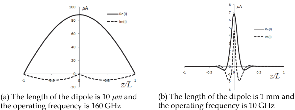
Fig. 8. Current distributions along carbon nanotube dipole antennas due to a unity voltage source.
