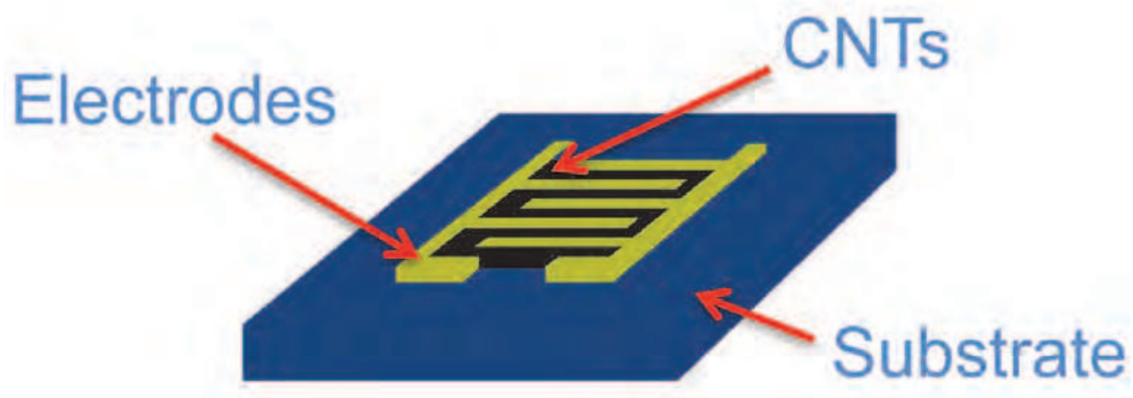
Fig. 1. Sketch of a typical prototype of CNTs-based radiation detector where the nanotubes are grown in between two interdigitated electrodes.
