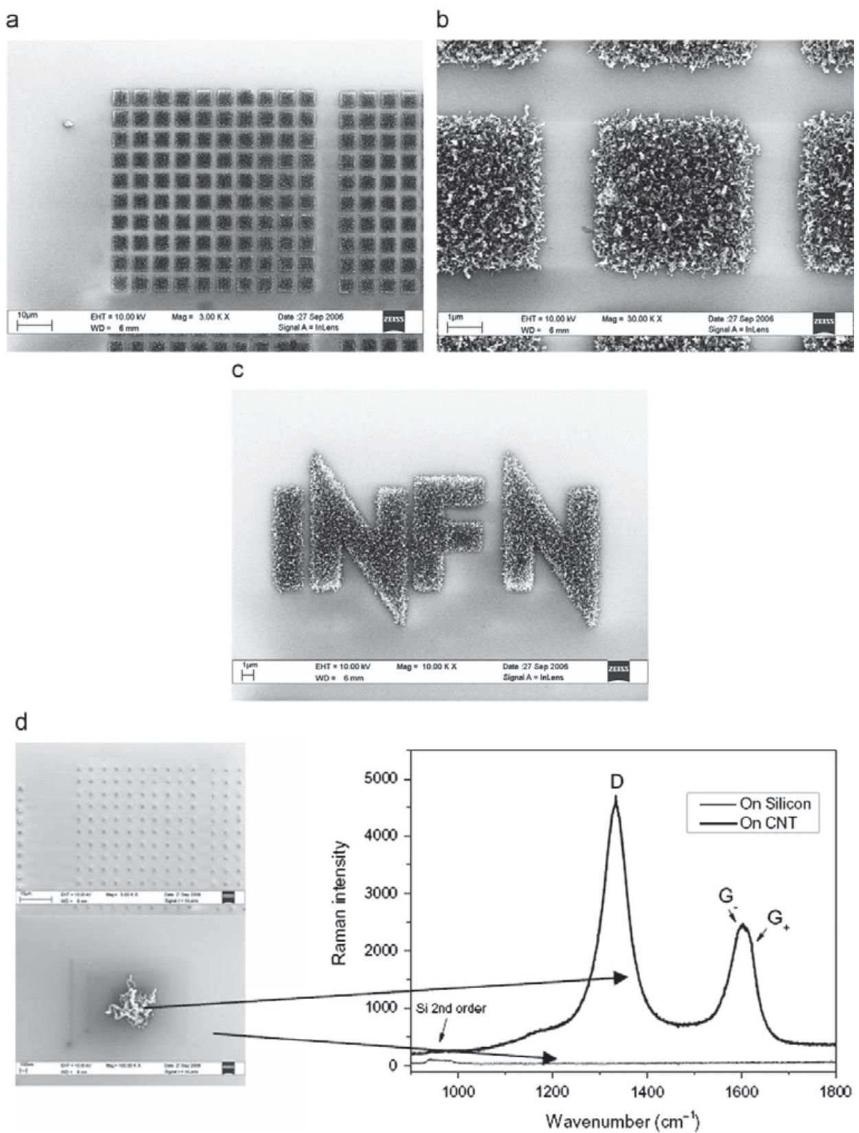
Fig. 9. a) a square CNT matrix of 10x10 pixels 4x4 mm 2 obtained with a lift-off process on lithographed mask; b) individual 2x2 µm 2 CNT pixel; c) the INFN logo made of CNT in micrometric scale; d) Raman image of CNT and silicon substrate
