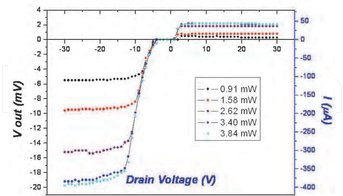
Fig. 6. The I-V plot related to a continuous laser beam, 650 nm wavelength, at different power.
