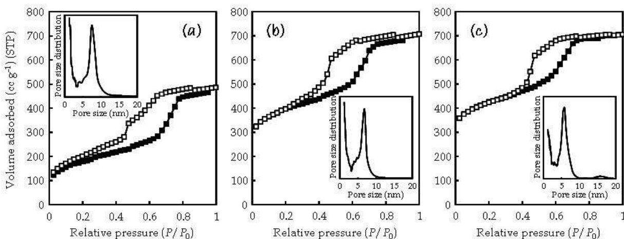
Fig. 7. \text{N}_2 adsorption/desorption isotherms and pore size distribution (inset) for carbonized COU-1. The carbonization temperatures were (a) 400 °C, (b) 600 °C, and (c) 800 °C. (Tanaka et al., 2005)
