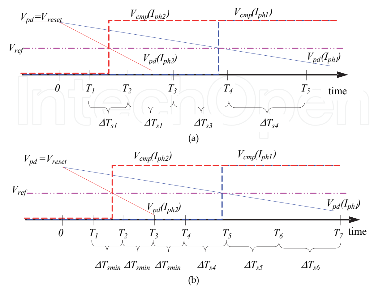
Fig. 6. Sampling in (a) logarithmic interval times (b) linear-logarithmic interval times
