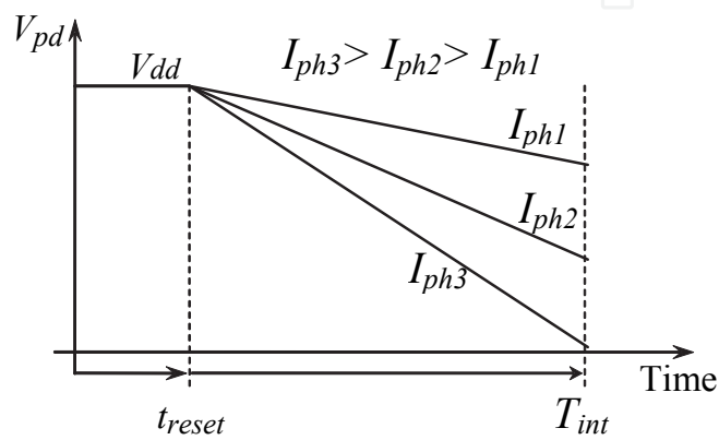
Fig. 1. Photodiode operating in integration mode
