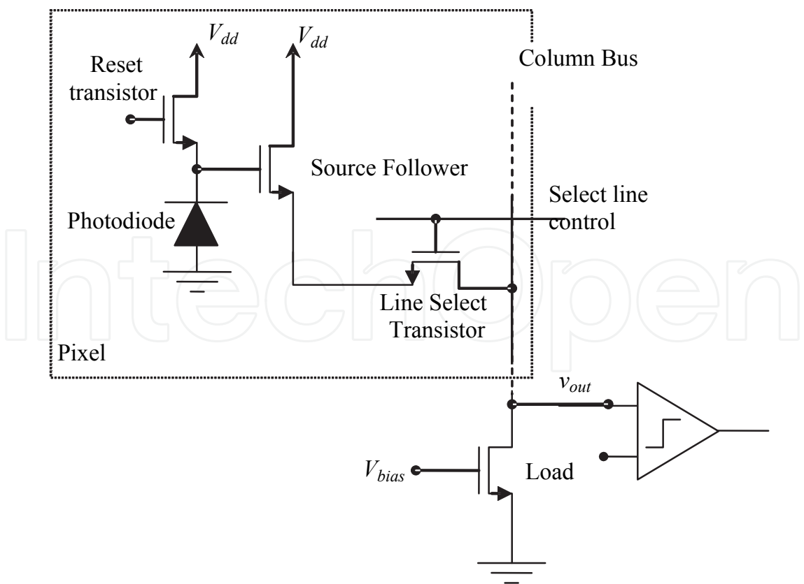
Fig. 14. A different architecture with high fill-factor for multisampling in time technique.
