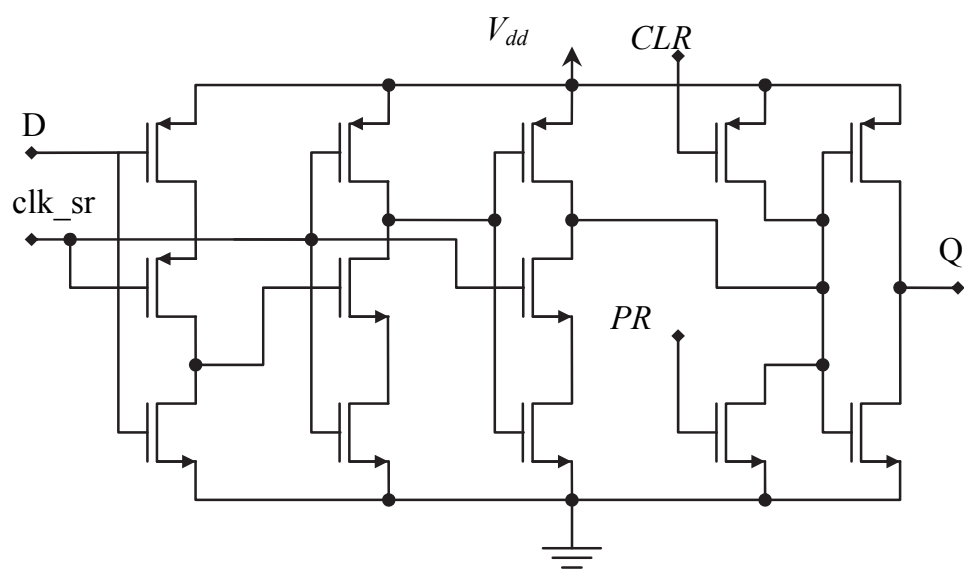
Fig. 12. Topology of dynamic D flip-flop with preset and clear
