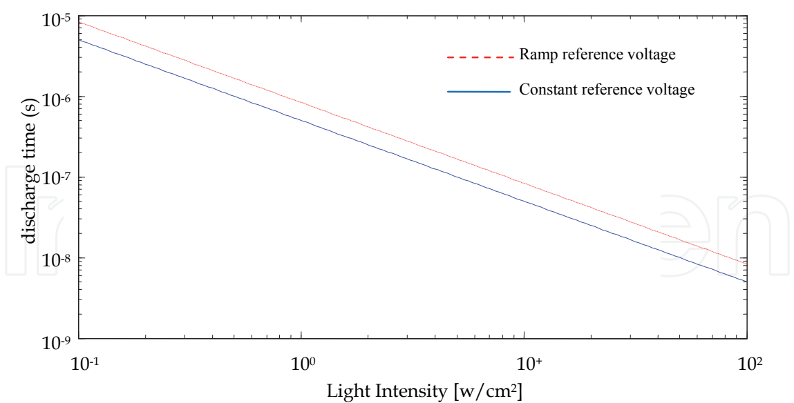
Fig. 4. Discharge time characteristic
