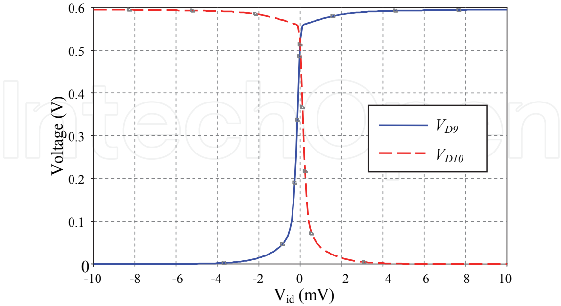
Fig. 11. Output voltage of comparator in track stage.
