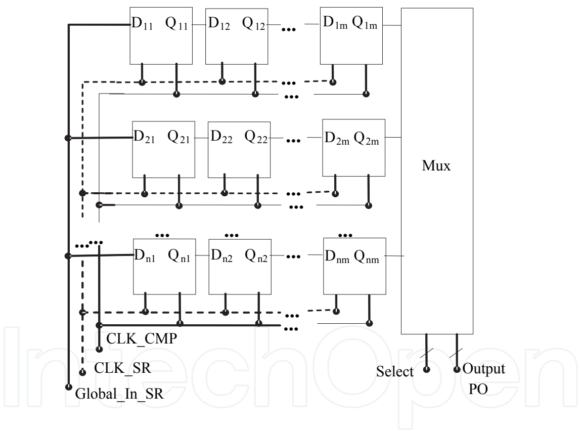
Fig. 8. Array block diagram
