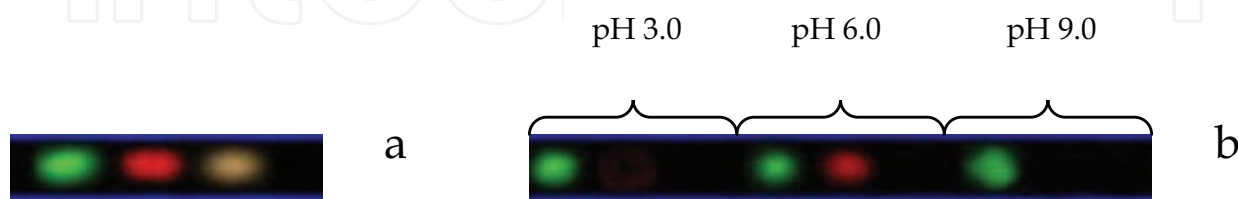
Fig. 6. Visualization of the proteins having different pI values and labelled with semiconductor nanocrystals under UV-source. The individual proteins before washing with the buffer solution (a) and retention of cytochrome C, myoglobine and pepsin on silicon-strips coated with poly -ANI-co-3-ABA by precipitation polymerization (b). The correspondence between the spot colour and individual proteins is shown in the table 2.
