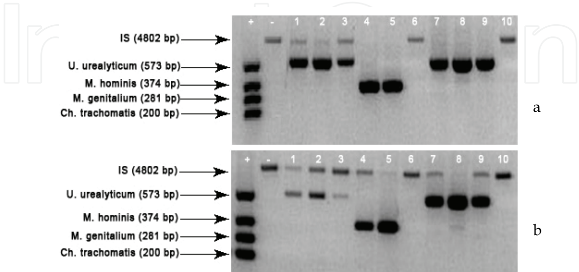
Fig. 9. PCR detection of Chlamydia trachomatis , Ureaplasma urealyticum , Mycoplasma hominis , and Mycoplasma genitalium in the randomly selected urinogenitalic smears from 10 patients (using the same samples as in the Figure 8). The results of the electrophoresis in 2% agarose gel. Isolation of DNA was carried out using the standard procedure developed by Diatom TM DNA Prep 100 Kit (IsoGen, Inc, Russia) (row a) and the cartridges packed with the developed PANI-coated adsorbent (row b). The arrows show the location of PCR fragments relating to internal standard (4802 bp), U. urealyticum (573 bp), M. hominis (374 bp), M. genitalium (281 bp), and Ch. trachomatis (200 bp).
