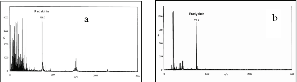
Fig. 7. MS spectra of peptide standards on a silicon strip modified with PANI-PABA with (a) and without an addition of CHCA as matrix (b).
