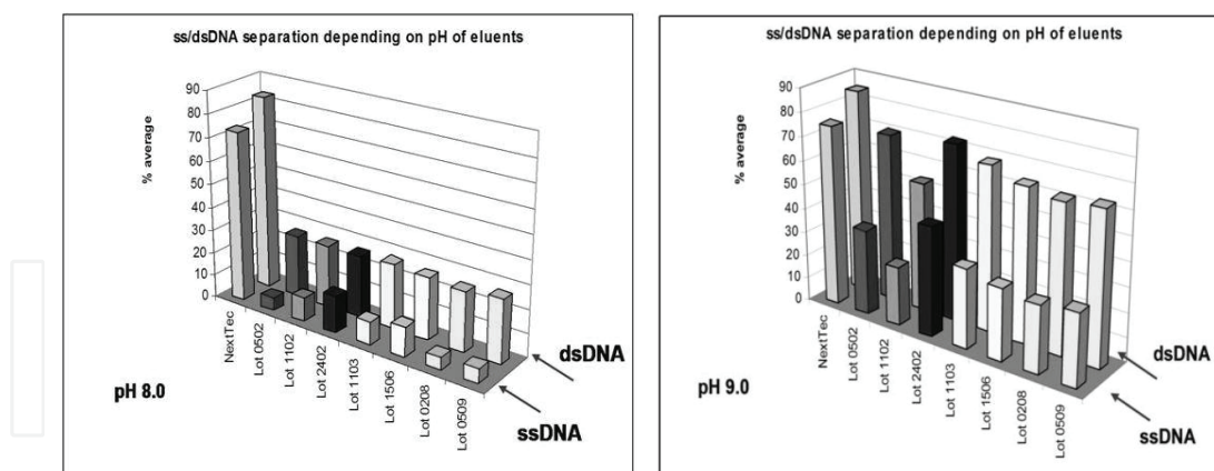
Fig. 5. Separation of ssDNA and dsDNA depending on pH of medium using iso -PSA-PANI-coated adsorbent.
