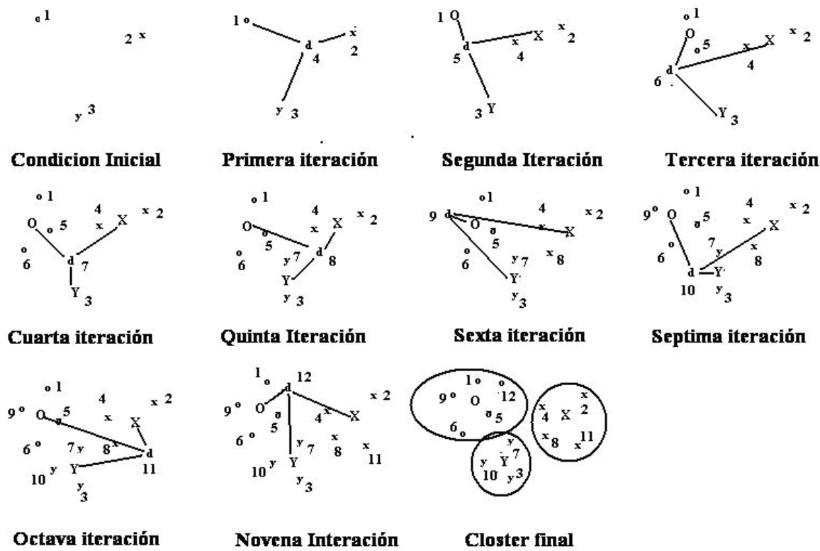
Fig. 3. Illustration of K-Means algorithm for M3.
