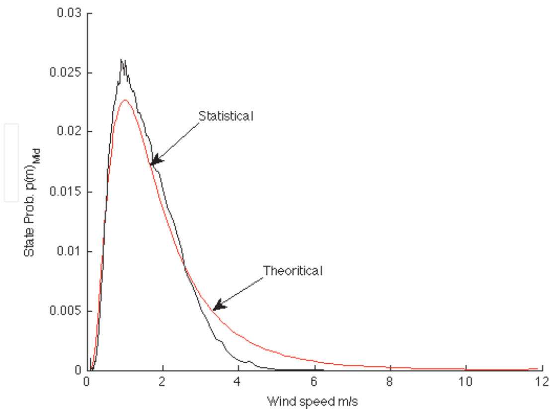
Fig. 20. Lognormal state probabilities ( M = 128 ) for medium frequency wind signal.
