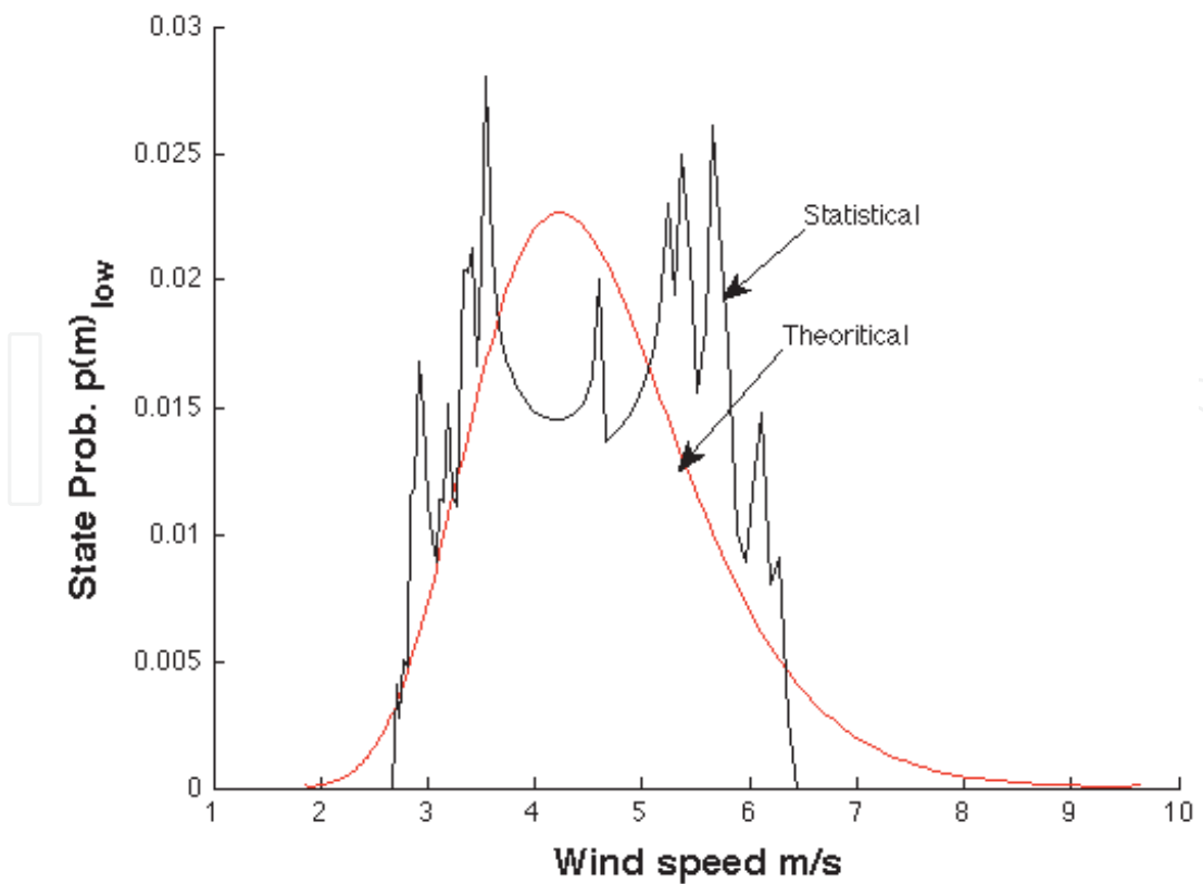
Fig. 21. Lognormal state probabilities ( M = 128 ) for low frequency wind signal.
