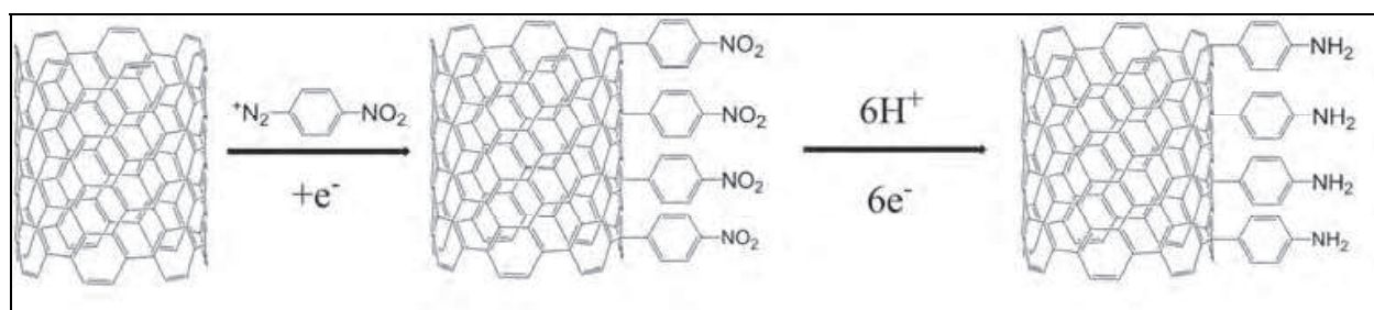
Fig. 3. Schematic for the electrochemical modification of CNTs.
