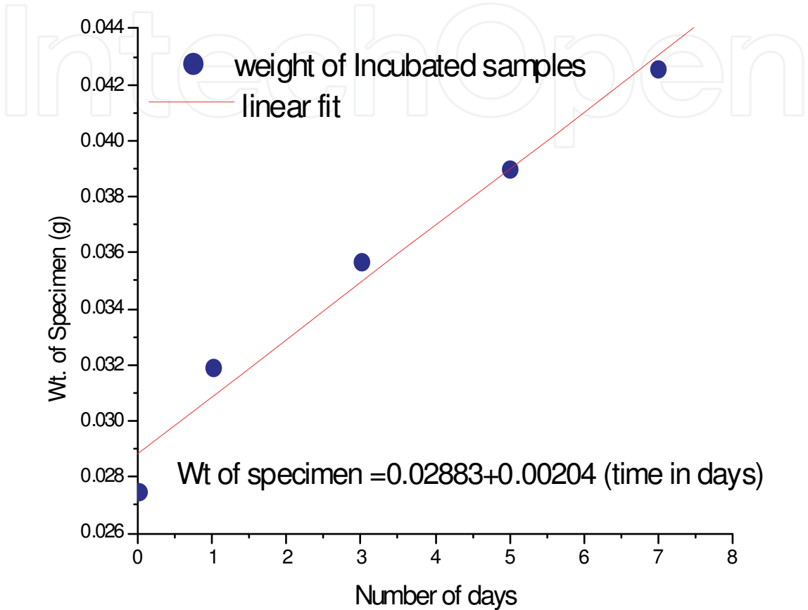
Fig. 5. Hydroxyapatite coating on UHMWPE/CNT composite with time during SBF test.
