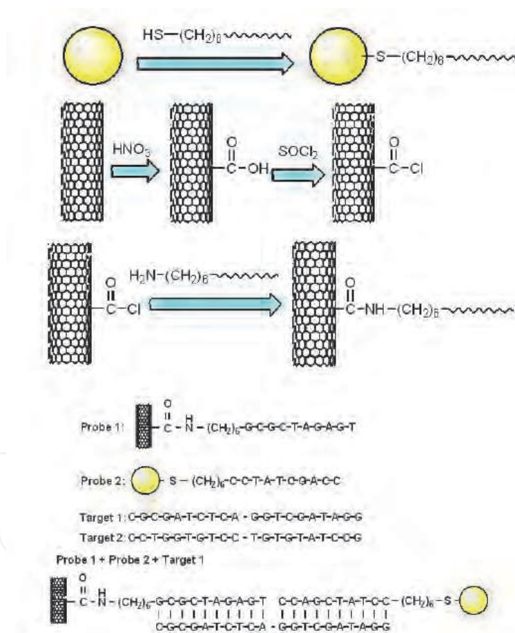
Scheme 2. Surface functionalization with oligonucleotide, and subsequent addition of target oligonucleotide to form CNT-QD assembly. Target 1, complementary DNA; target 2, non-complementary DNA. (With permission from American Chemical Society)
