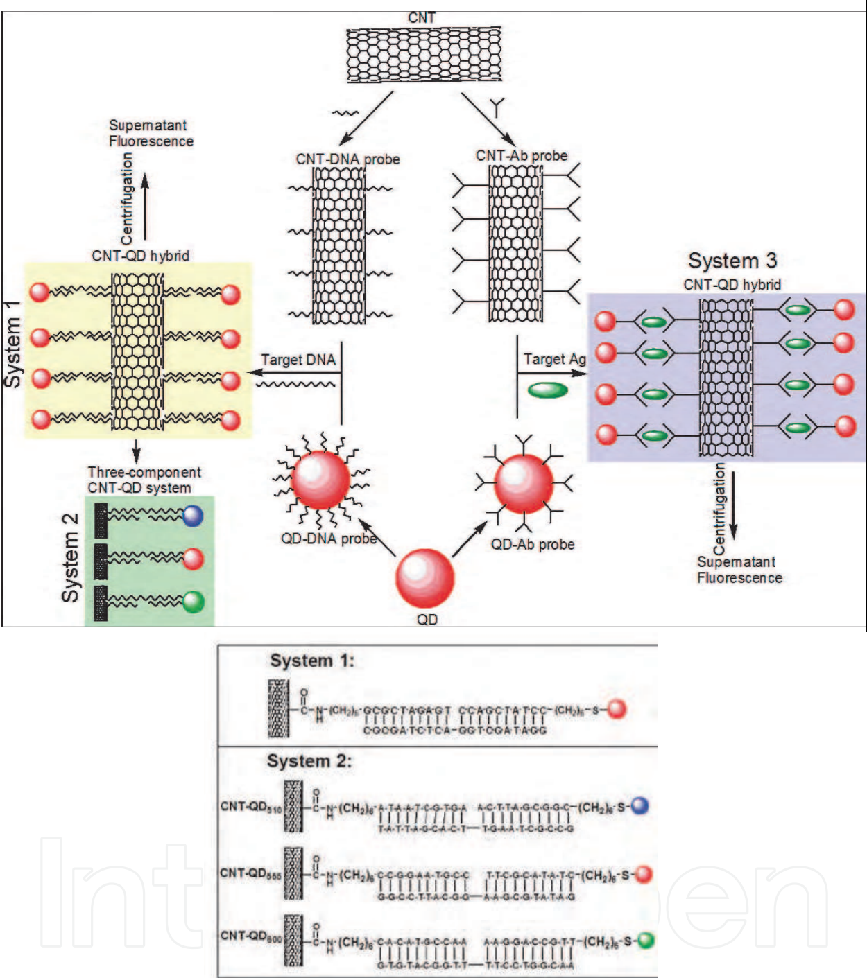
Scheme 3. Surface Functionalization of CNT (or QD) with Oligonucleotide/ Antibody (Ab), Forming aCNT-DNA (or -Ab) Probe and QD-DNA (or -Ab) Probe, and Subsequent Addition of Target Oligonucleotide (or Antigen) to Form a CNT-QD Assembly a (a The unbound QD probe was obtained by simple centrifugation separation, and the supernatant fluorescence intensity of QDs was monitored by spectrofluorometer. (System 1) Formation of CNT-QD hybrid in the presence of complementary DNA target. (System 2) Three-component CNT-QD system with the purpose to detect three different DNA targets simultaneously. (System 3) CNT-QD protein detection system based on antigen-antibody immunoreaction.) (With permission from American Chemical Society)
