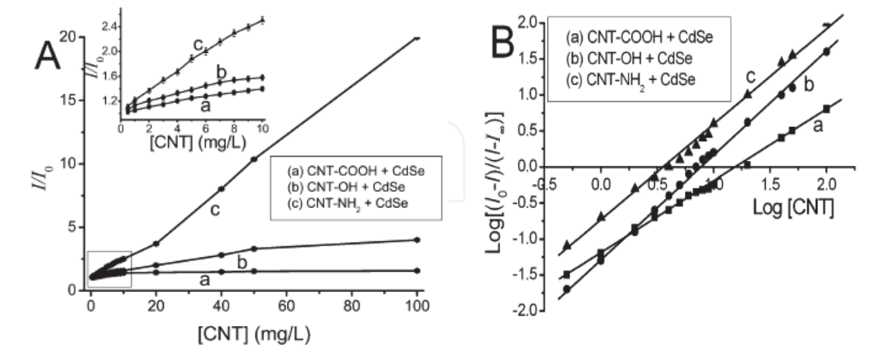
Fig. 14. (A) Stern-Volmer plot and (B) double-logarithmic plot for CdSe PL quenching by CNT with different concentration. (With permission from American Chemical Society)
