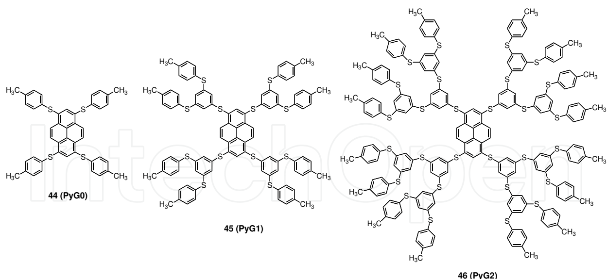
Fig. 7. Polythiophenylene-functionalized pyrene-cored light emitting dendrimers ( 44-46 ).
