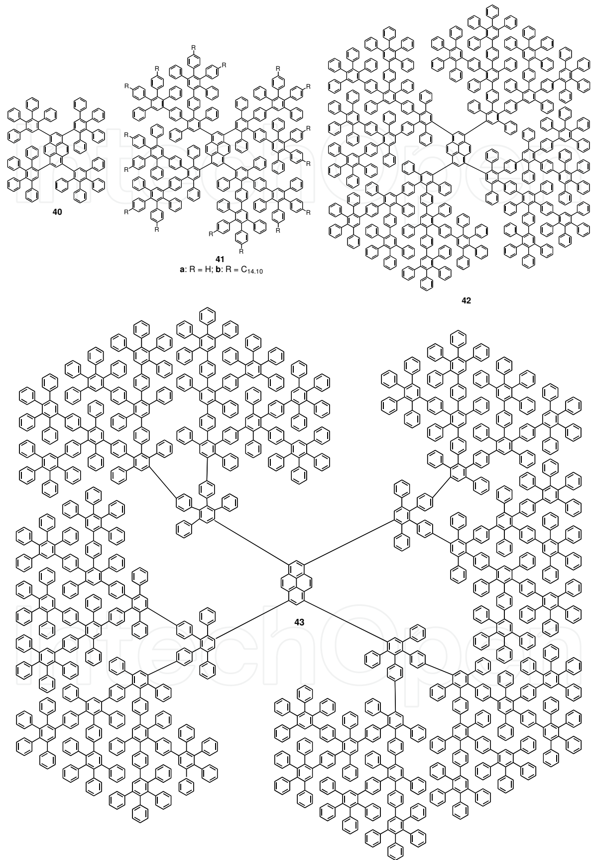
Fig. 6. Polyphenylene-functionalized pyrene-core light emitting dendrimers (40-43).
