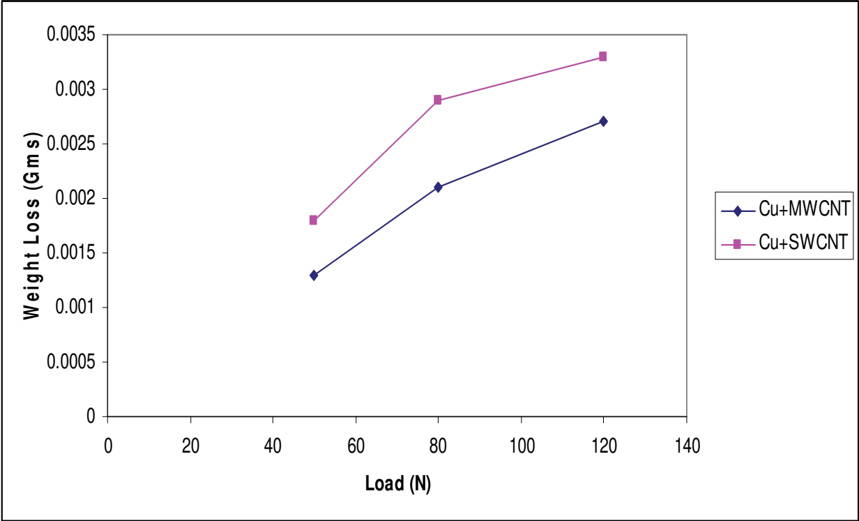
Fig. 13. Load Vs Weight loss
