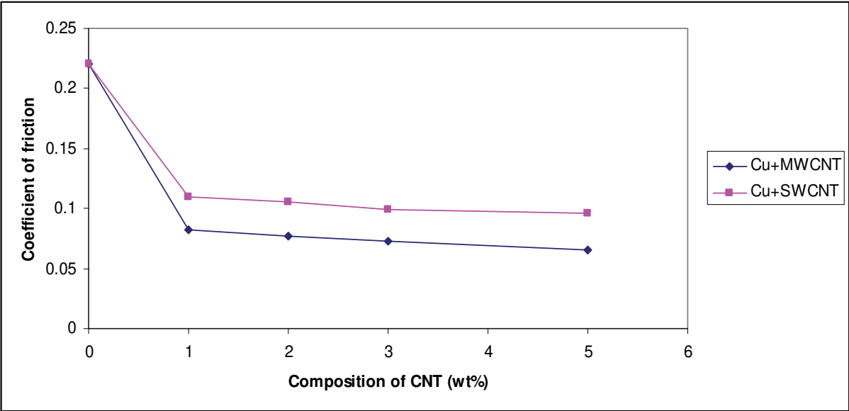
Fig. 10. CNT Composition Vs Coefficient of Friction of Cu, Cu/MWCNT & Cu/SWCNT
