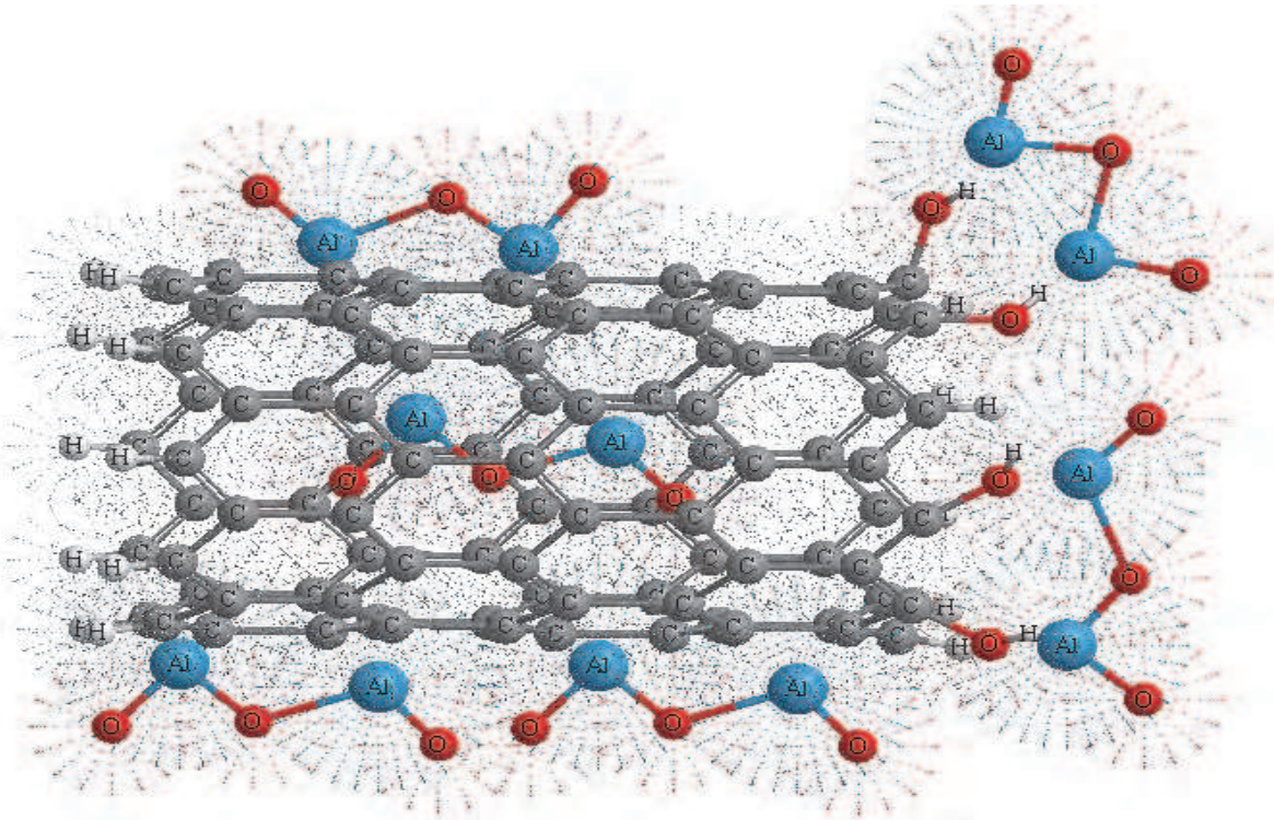
Fig. 5. Structural representative of possible interaction between \text{Al}_2\text{O}_3 and carbon nanotube in MWCNT/ \text{Al}_2\text{O}_3 nanocomposite.
