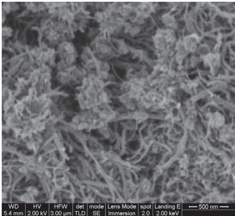
Fig. 6. Field emission scanning electron microscope (FESEM) of MWCNT/ Al 2 O 3 nanocomposite
