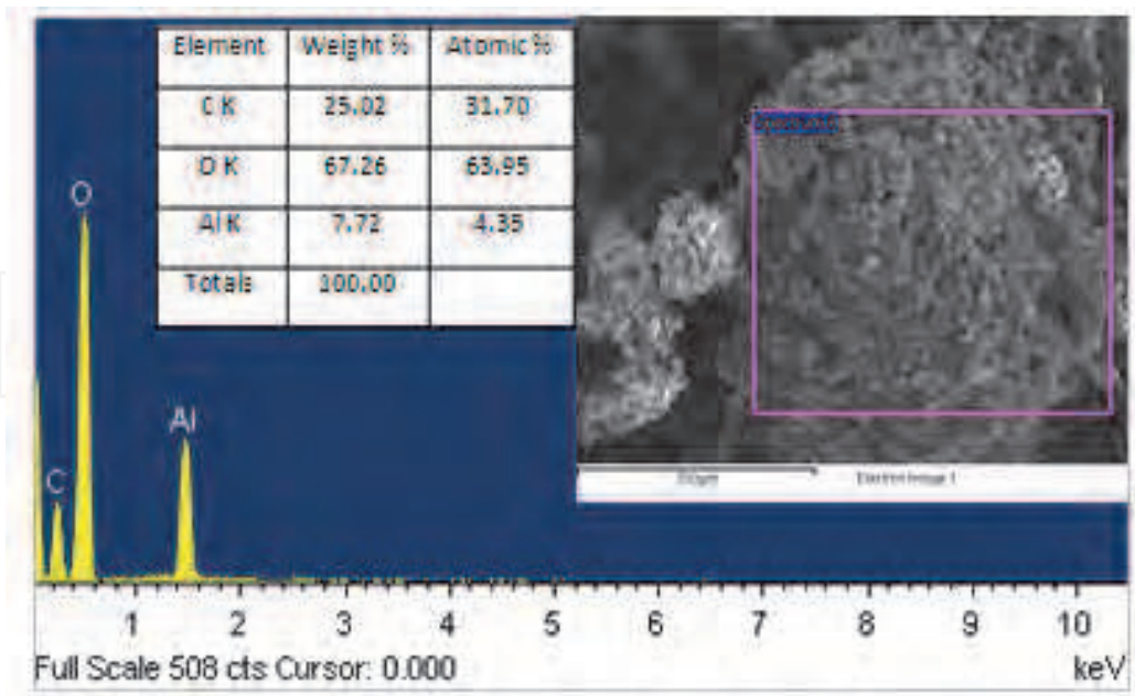
Fig. 7. Energy dispersive X-ray (EDX) spectrum of the area indicated in the Inset: low magnification scanning electron microscope (SEM) of MWCNT/ Al 2 O 3 nanocomposite; Inset: Table presents the atomic ratio, percentage of the components in the nanocomposite.
