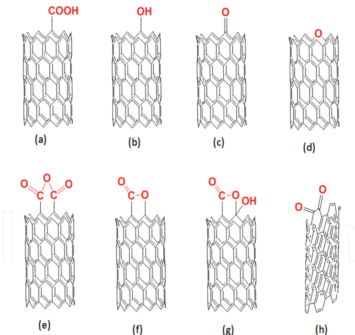
Fig. 1. Possible structures of oxygen-containing groups on the carbon nanotube surface
