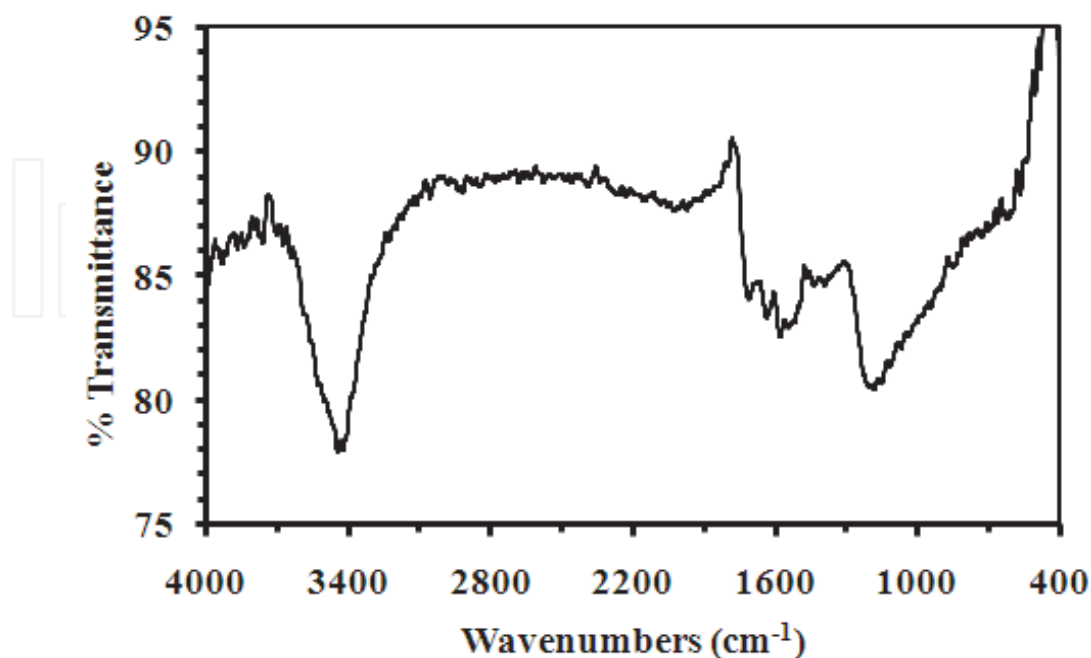
Fig. 2. FTIR spectra of MWCNT oxidized with mixtures of \text{H}_2\text{SO}_4/\text{HNO}_3 at 100 °C.
