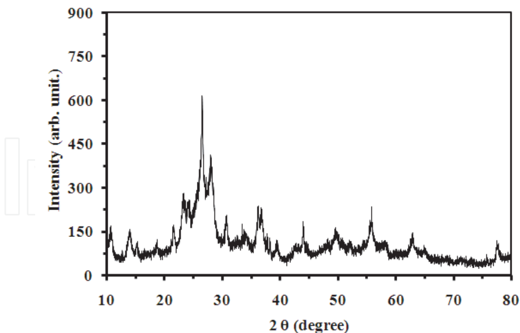
Fig. 8. XRD patterns of MWCNT/WO 3 nanocomposite.
