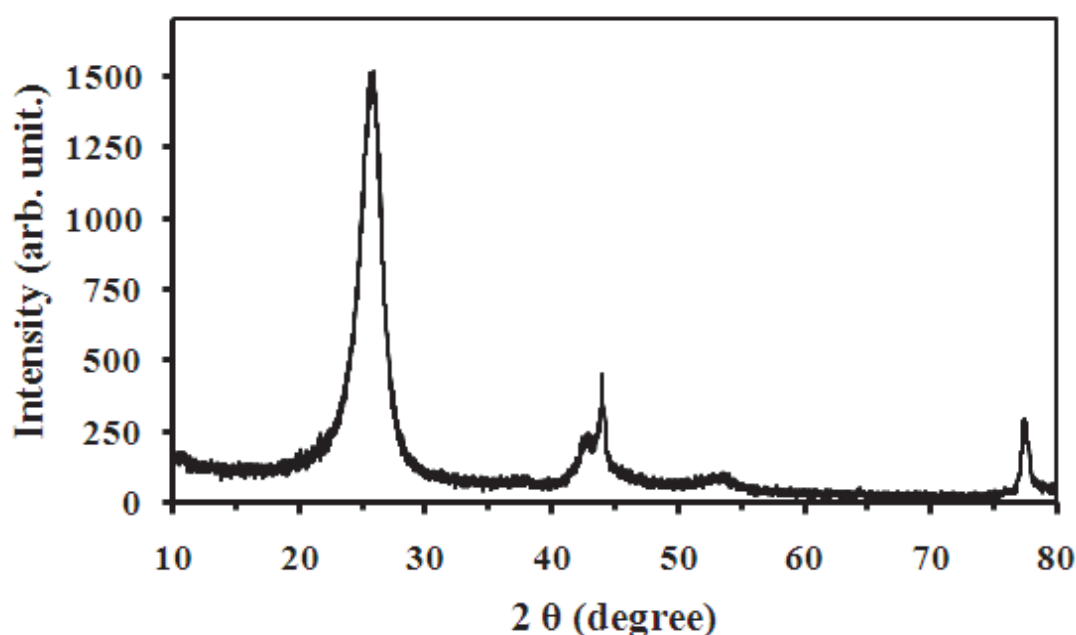
Fig. 3. XRD patterns of MWCNT oxidized with \text{HNO}_3 at 120^\circ\text{C}
