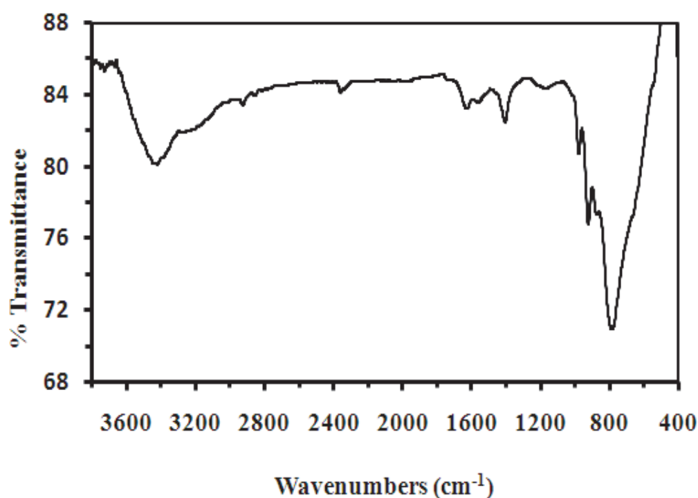
Fig. 9. FTIR spectra of MWCNT/WO 3 nanocomposite.
