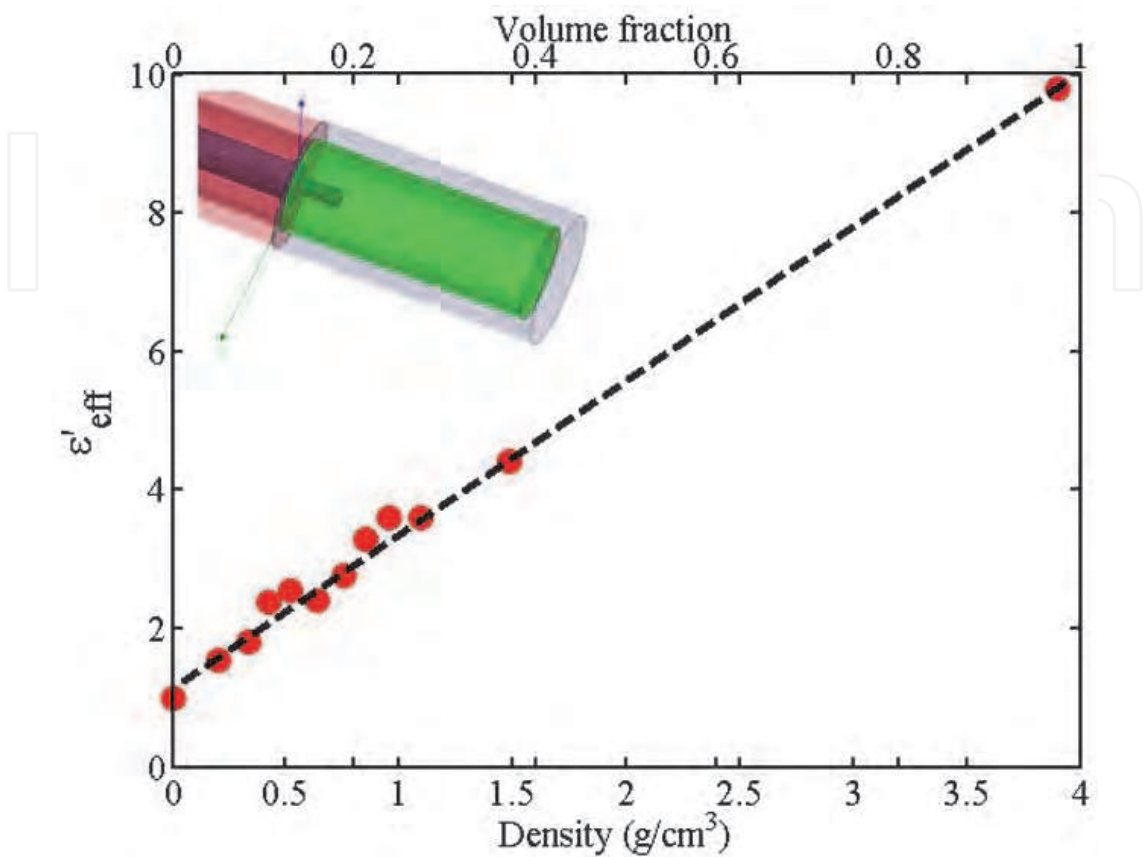
Fig. 6. Variation of extracted effective dielectric constant of pure Al 2 O 3 versus density or the volume fraction at 3 GHz using the test setup shown in Fig. 1. The last point is the common accepted value \epsilon'_{eff} = 9.8 at a bulk density of 3.9 g/cm 3 for pure alumina.
