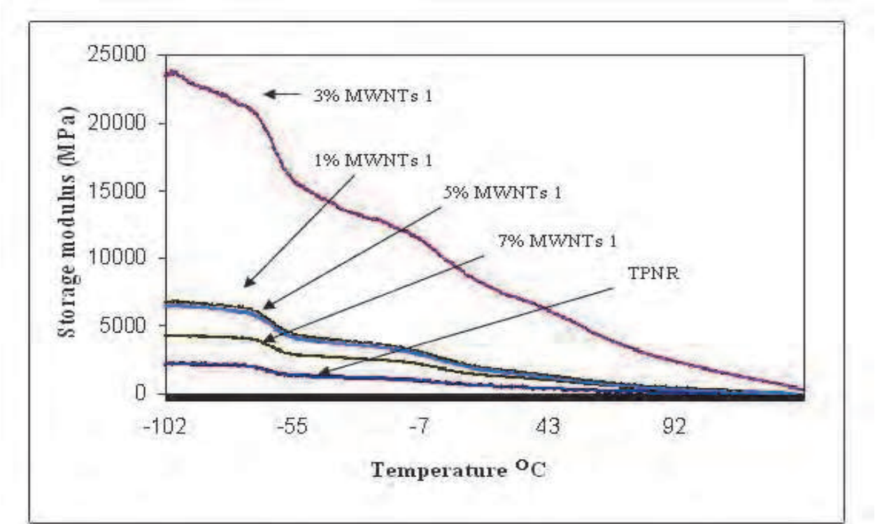
Fig. 5. Storage modulus of TPNR and TPNR/MWNTs 1 nanocomposites.
