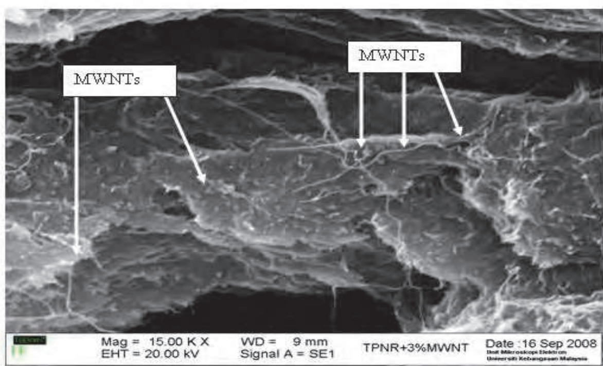
Fig. 21. SEM micrograph of TPNR with 3 % MWNTs 1.
