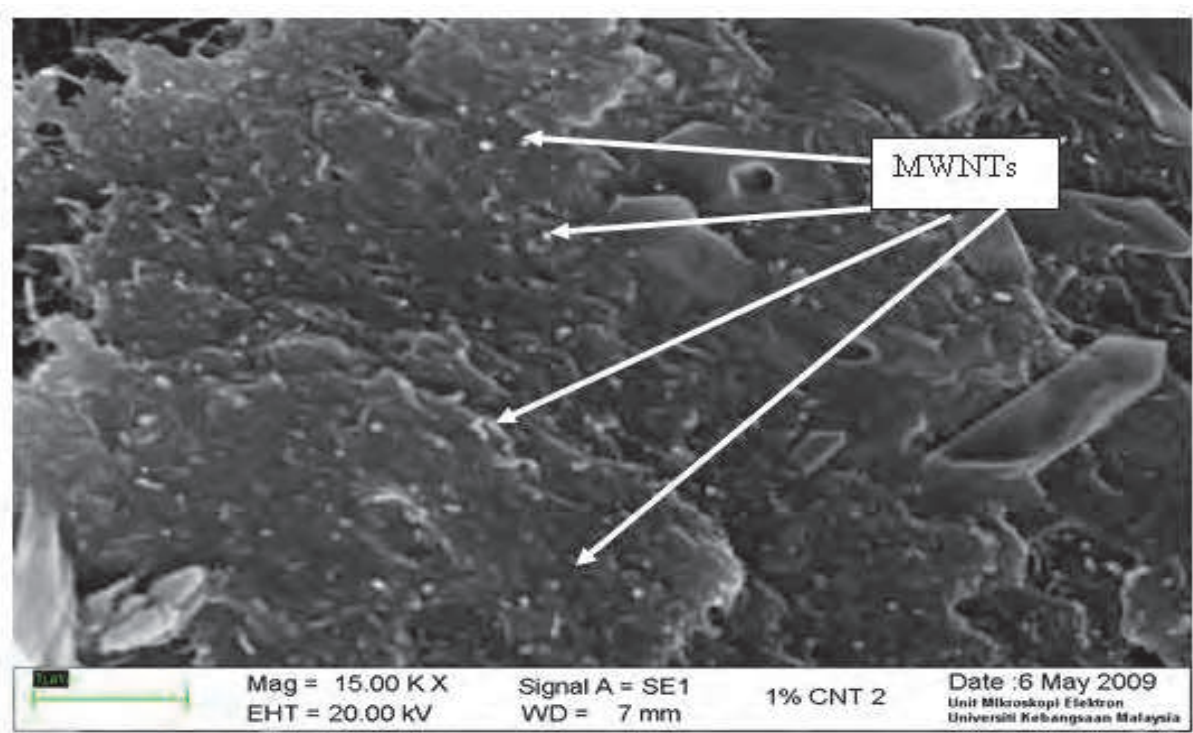
Fig. 24. SEM micrograph of TPNR with 1% MWNTs 2.
