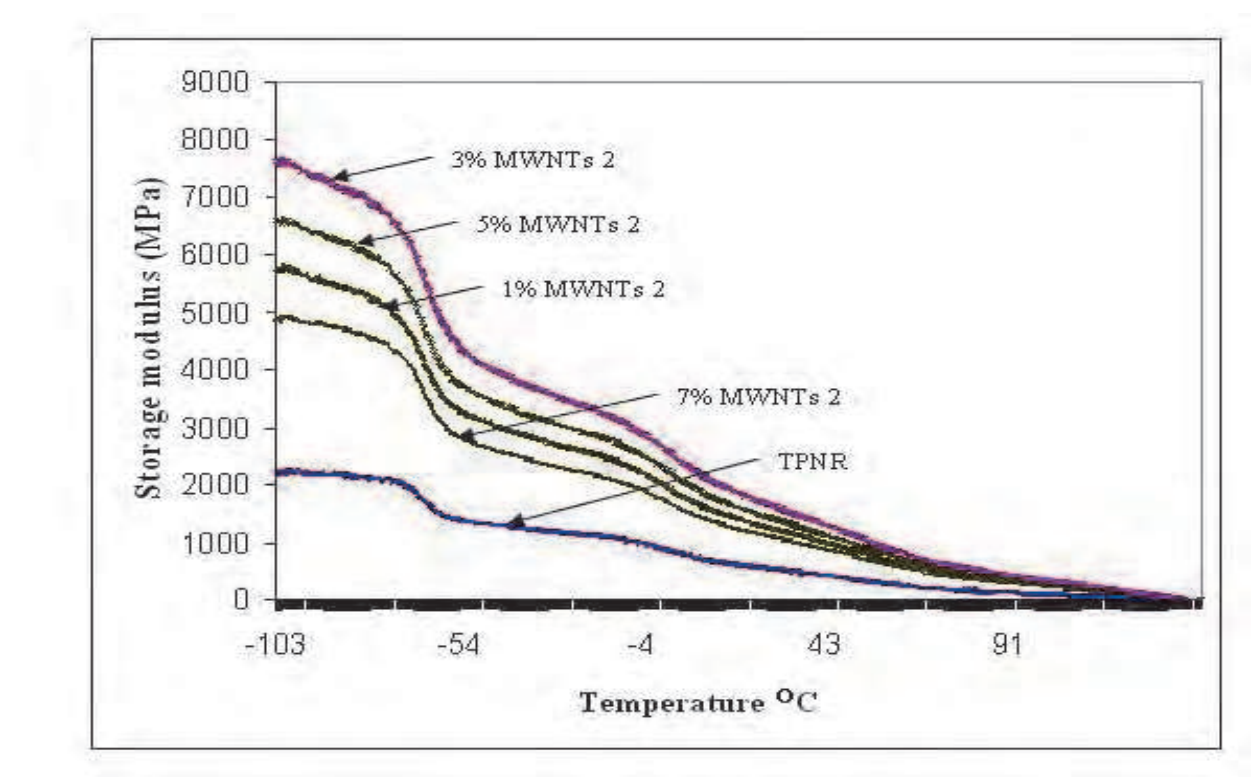
Fig. 6. Storage modulus of TPNR and TPNR/MWNTs 2 nanocomposites.
