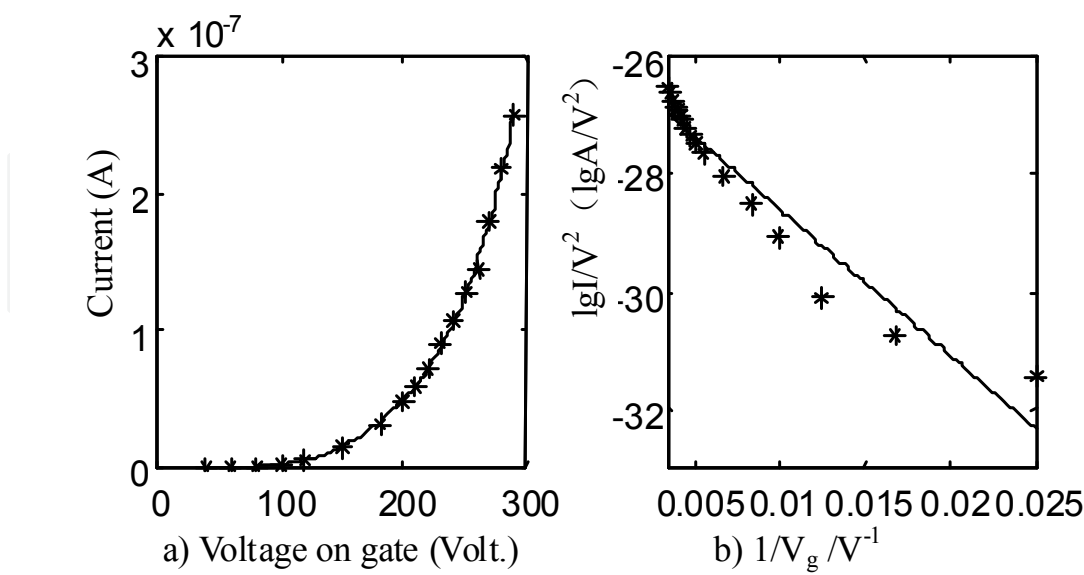
Fig. 12. I-V curve and F-N plot
