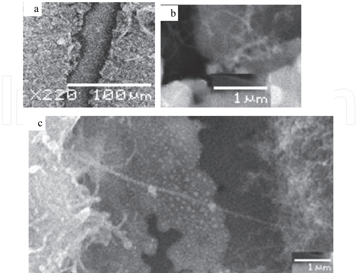
Fig. 1. (a) a trench etched with laser; (b) carbon nanotube on the edge of trench; (c) a carbon nanotube with the length of 5μm
