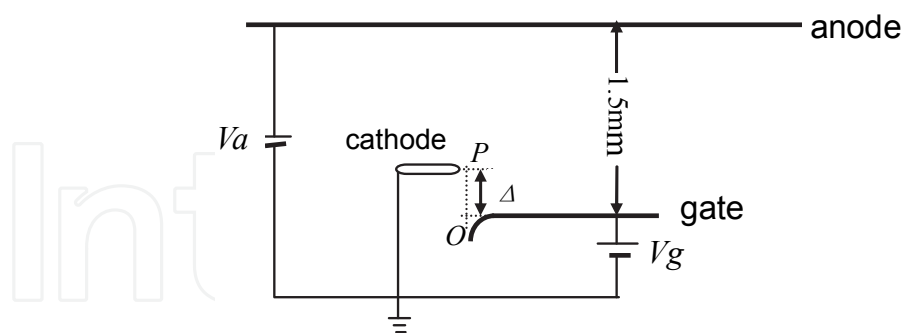
Fig. 5. Model of electric structure
