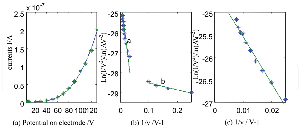
Fig. 2. (a). Emitting current vs. Voltage, (b). F-N plot (Potential ranged from 4V~130V) (c). F-N plot (Potential ranged from 40V~130V)
