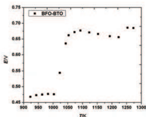
Fig. 7. Temperature dependence of EMF for \text{Bi}_{0.90}\text{Ba}_{0.10}\text{Fe}_{0.90}\text{Ti}_{0.10}\text{O}_3
