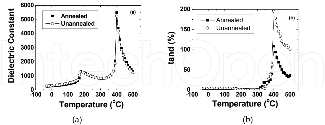
Fig. 8. Temperature dependence of dielectric constant and loss for KNN. (a) Dielectric constant and (b) Dielectric loss.
