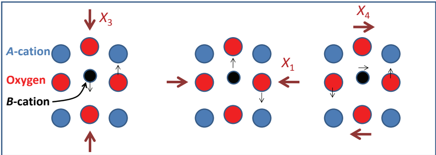
Fig. 1. Understanding the relationship between the crystal structure and property is crucial. Given example is for tetragonal (space group P4mm ) perovskite single crystal. Classical examples are \text{BaTiO}_3 and \text{PbTiO}_3 . In the absence of external stimuli polarization appears along the c -axis. Application of stress X_1 , X_3 and X_4 in turn results in the illustrated changes in polarization. Figure after M. Dove (Dove, 2003).
