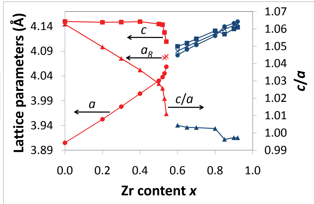
Fig. 8. Room-temperature tetragonal (space group P4mm ) and pseudo-tetragonal (space group Cm ) a (filled spheres) and c axis (filled squares) parameters and the c/a axis ratio (filled triangles). Lattice parameter, a_R , for rhombohedral phase (space group R3c ) is indicated by crosses. In the case of the monoclinic Cm phase (structure slightly deviates from the tetragonal structure) the average of the a and b axes were divided by \sqrt{2} , whereas a_R = \frac{1}{3}\sqrt{3a_H^2 + (c_H/2)^2} , where a_H and c_H are the hexagonal lattice parameters. The data indicated by black colour are from. refs. (Frantti et al., 2000; 2002; 2003) and the data indicated by blue colour are from. ref. (Yokota, 2009).
