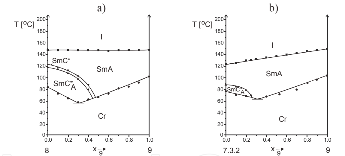
Fig. 15. Phase diagrams of bicomponent mixtures of compounds with alkyl group with destabilization of SmC*_A phase - weaker in system 8-9 (a), and stronger in system 7.3.2-9 (b)
