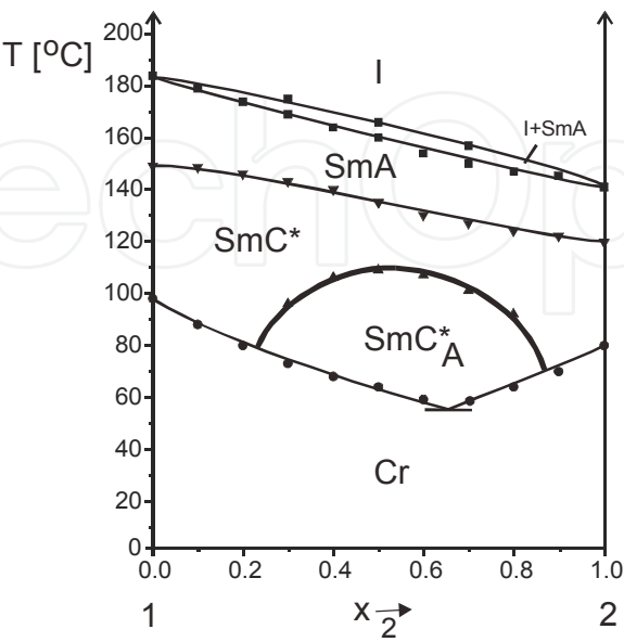
Fig. 2. Phase diagram of the system 1-2 [Dąbrowski 2000].
