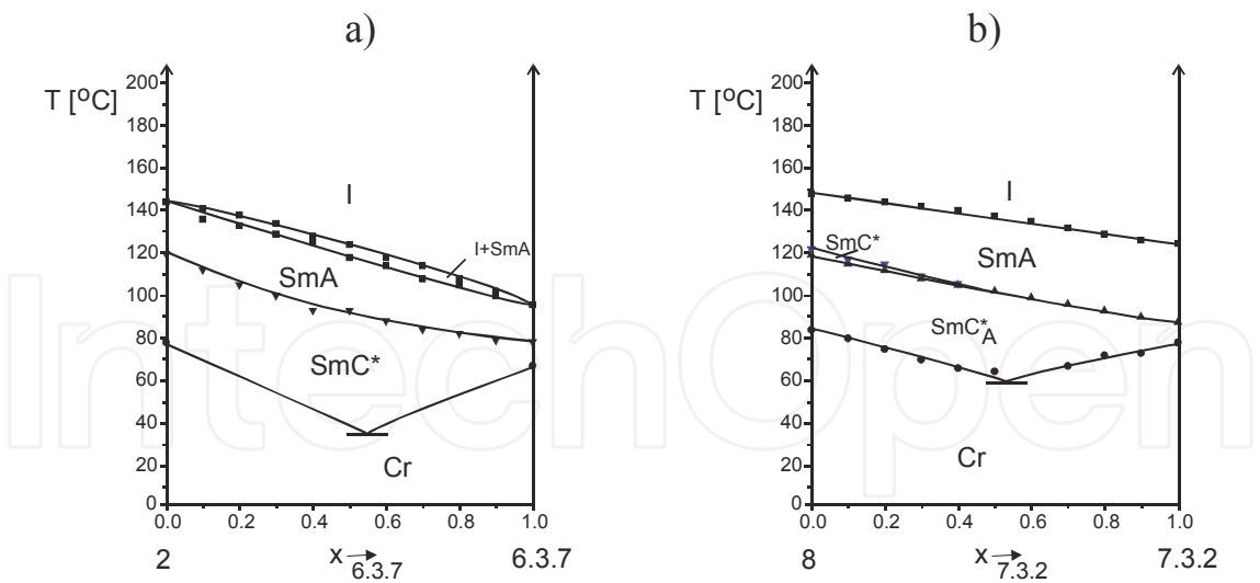
Fig. 14. Phase diagrams of bicomponent mixtures of compounds with alkyl group with additive miscibility of SmC* phase - system 2-6.3.7 (a), and with additive miscibility of SmC*_A phase - system 8-7.3.2 (b)
