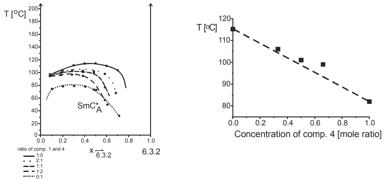
Fig. 13. The collective phase diagram showing curves corresponding to phase transition temperature from SmC*_A phase in mixtures of different concentration of compounds 1 and 4 (1:0, 2:1, 1:1, 1:2 and 0:1) with compound 6.3.2 (a), maximum temperature of SmC*_A existence versus concentration of compound 4 (b) [Tykarska et al. 2011]
