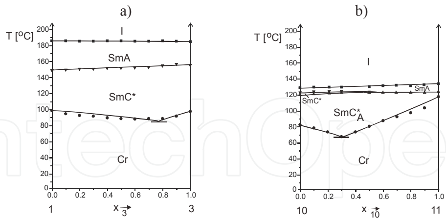
Fig. 16. Phase diagrams of bicomponent mixtures of compounds with fluoroalkyl group with additive miscibility of SmC* phase - system 1-3 (a), and with additive miscibility of SmC*A phase - system 10-11 (b)
