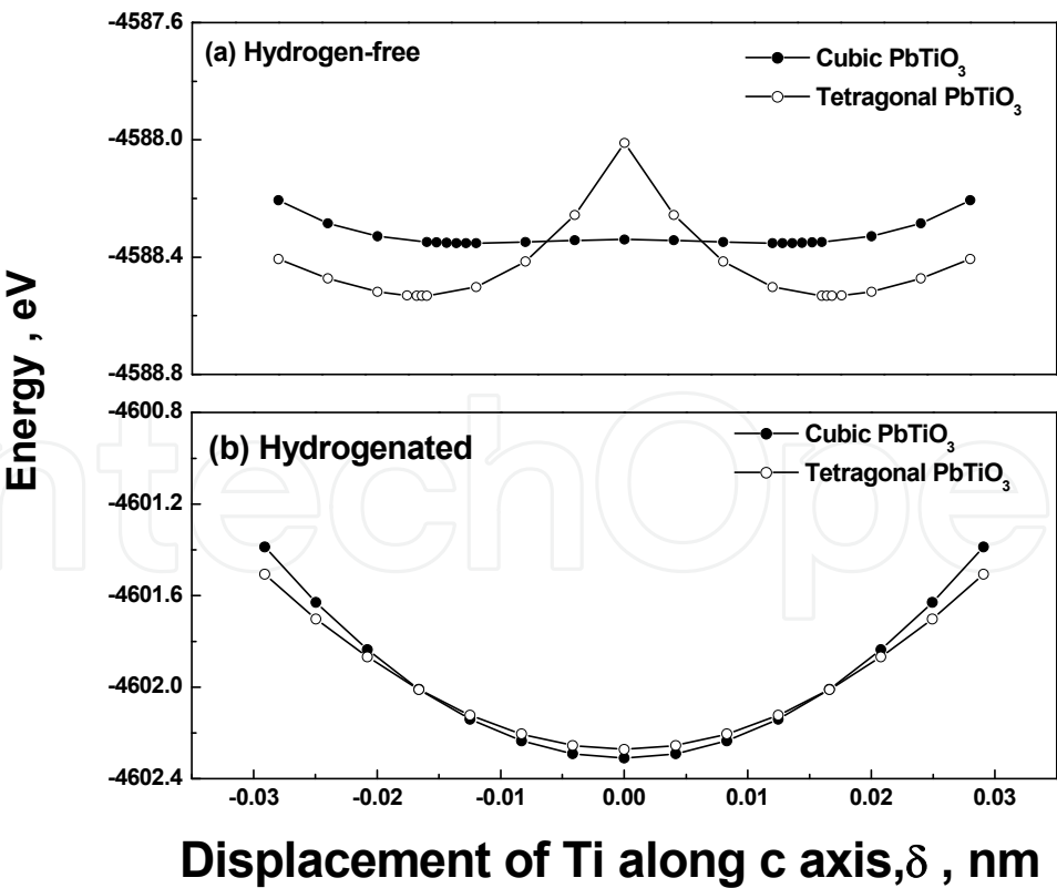
Fig. 6. Total energy vs. displacement of Ti along c axis, the original is the centre of the cell (a) hydrogen-free PbTiO 3 , (b) hydrogenated PbTiO 3 (Huang, et al., 2006)
