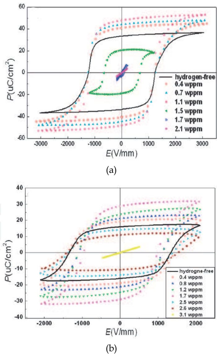
Fig. 2. The effects of hydrogen on hysteresis loops (a) PZT & (b) PZNT (Wu et al., 2010)
