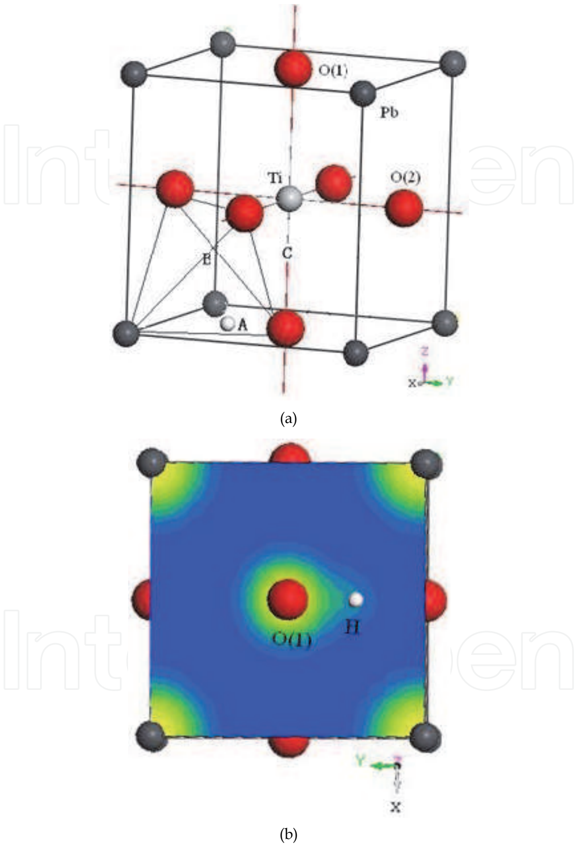
Fig. 5. Unit cell of tetragonal \text{PbTiO}_3 containing one hydrogen atom (a), and electronic clouds of XOY plane (b) (Huang, et al., 2006)
