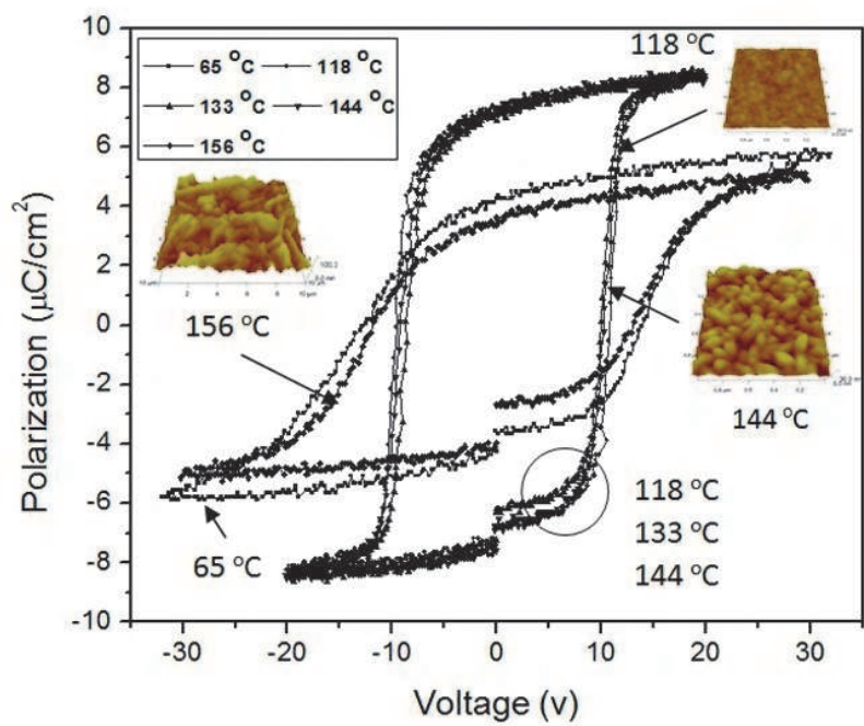
Fig. 17. The hysteresis loops of P(VDF-TrFE) FeCaps annealed at different temperatures. Reprinted from [Mao et al., 2010a] with permission.
