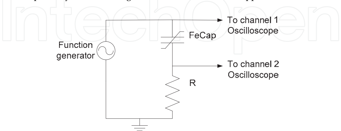
Fig. 8. The circuit schematic used to measure the currents in the switching and nonswitching transients using the PUND method.
