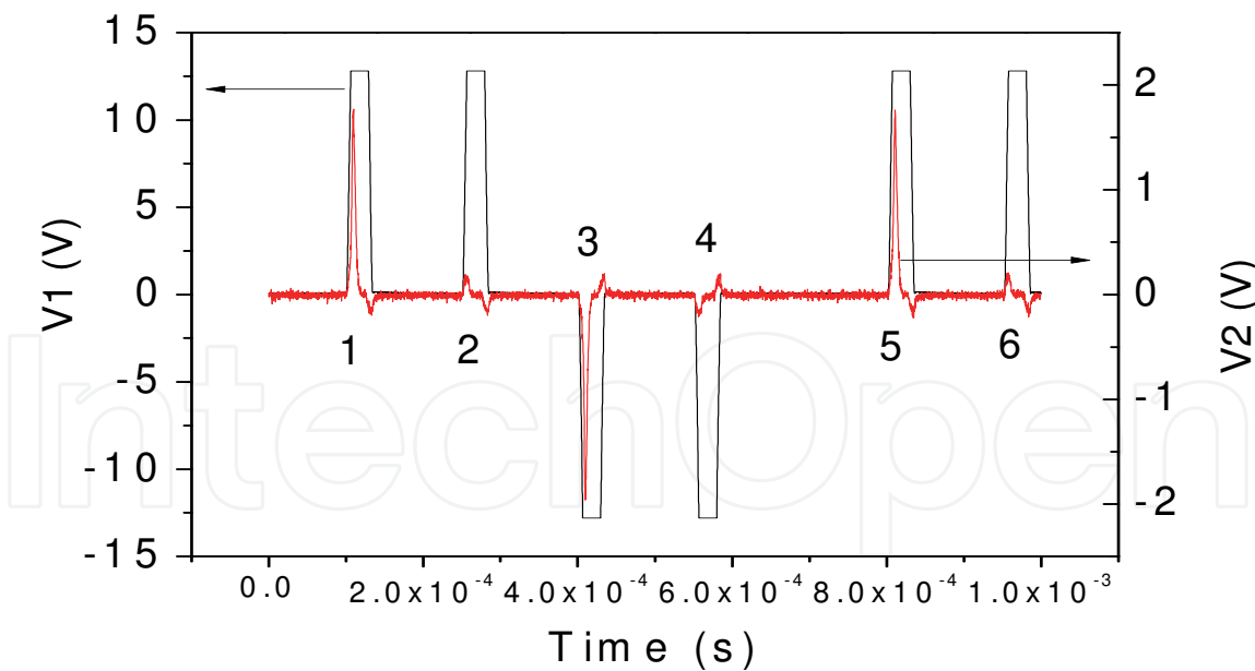
Fig. 9. The switching and nonswitching transient measurement of a P(VDF-TrFE) based FeCap using the PUND method.
